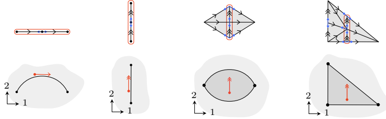
FIGURE 1.56. Highest frame vectors and axel vectors of framed regular 1-cells and 2-cells.
