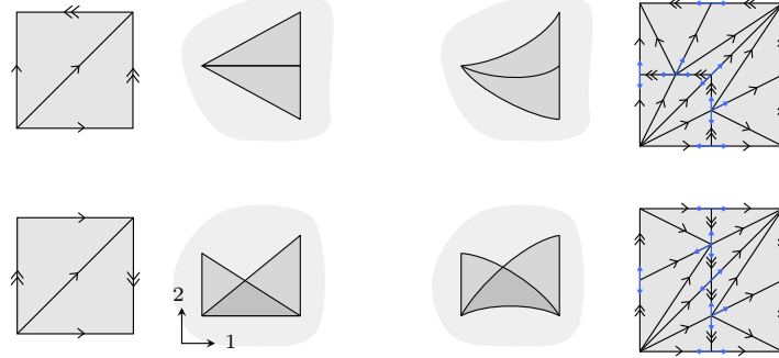
FIGURE 1.61. Framed simplicial complexes and their associated framed cell complexes.
