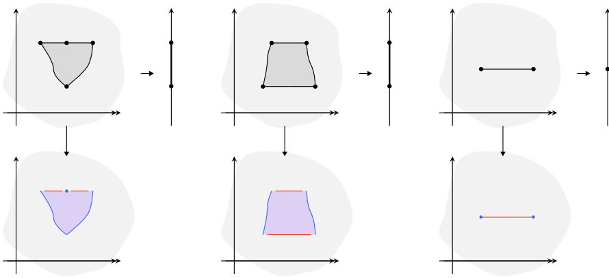
FIGURE 5.30. 2-Mesh cells.
