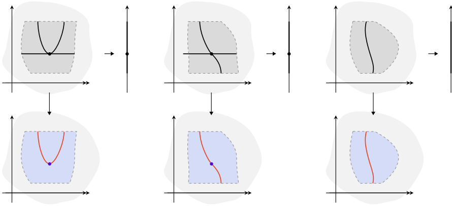
FIGURE 5.29. 2-Mesh singularities.
