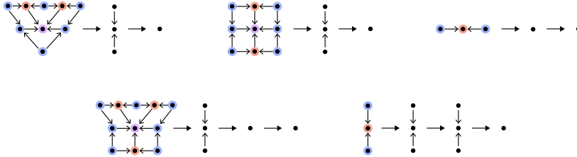
FIGURE 5.27. Truss singularities.
