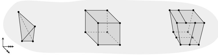
FIGURE 1.51. Framed 3-cells.
