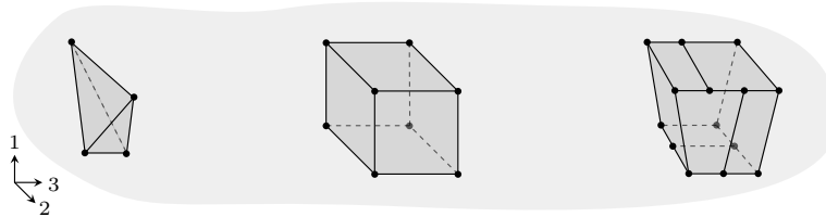
FIGURE 1.51. Simple framed 3-cells.
