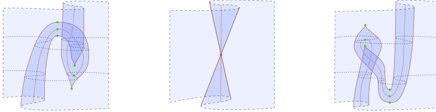
FIGURE 5.47. A manifold 4-diagram.
