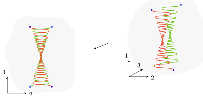
FIGURE 5.7. Nonlocal untameness.
