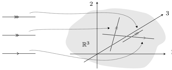
FIGURE 1.10. Framed realization of the 3-embedded framed 1-simplices.
