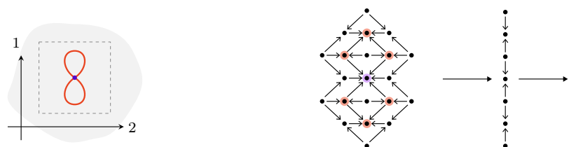
FIGURE 5.33. Normalized ambient stratified truss of the figure-8.
