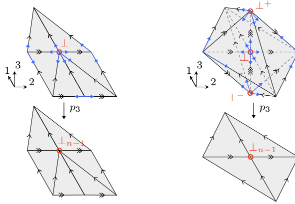
FIGURE 3.16. Framed section and spacer cells.
