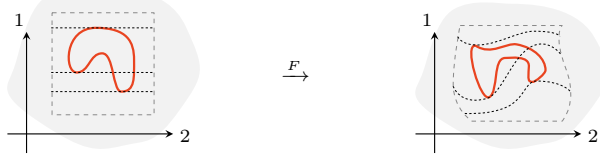
FIGURE 5.9. Non-framed stratified homeomorphism.
