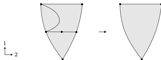
FIGURE I.6. A framed cell subdivision and a truss block subdivision.
