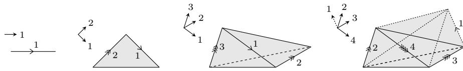
FIGURE 1.4. Framed simplices.
