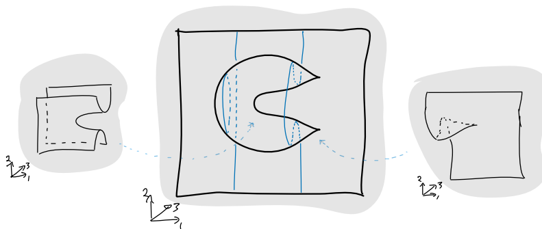
FIGURE 5.48. Two tangle singularities in a tame 2-tangle.
