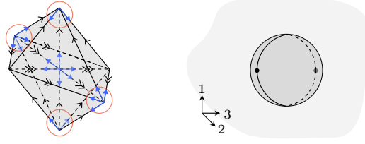
FIGURE 1.50. A framing of the simplicial complex underlying the regular 3-globe that does not yield a framed regular cell.
