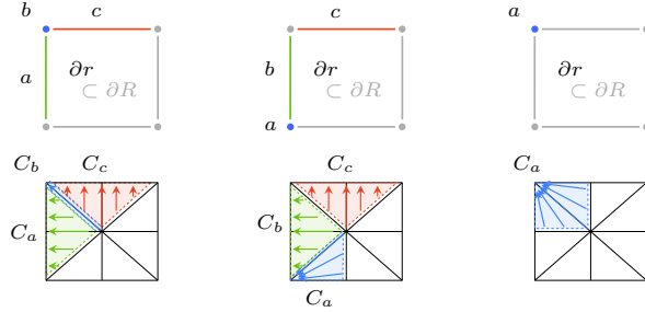
FIGURE 4.20. Catchment areas for cells and their decomposition into radial catchment paths.
