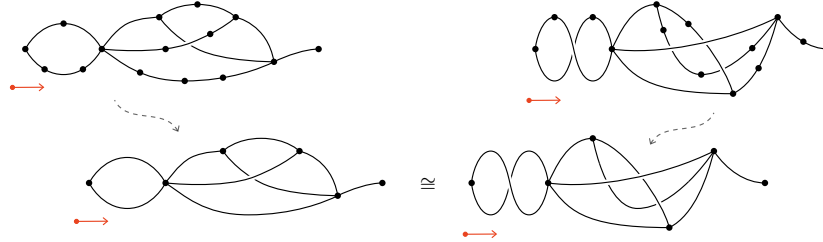
FIGURE 5.41. Decidability of framed homeomorphism for 1-DAGs.
