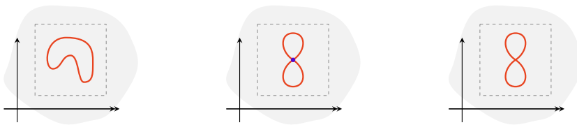
FIGURE 5.3. 2-Tame embeddings.
