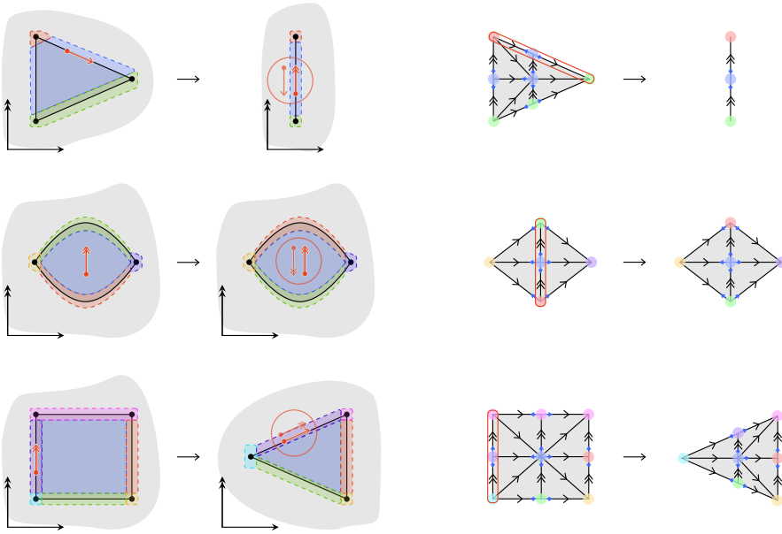
FIGURE 1.59. Cellular maps that are not framed.
