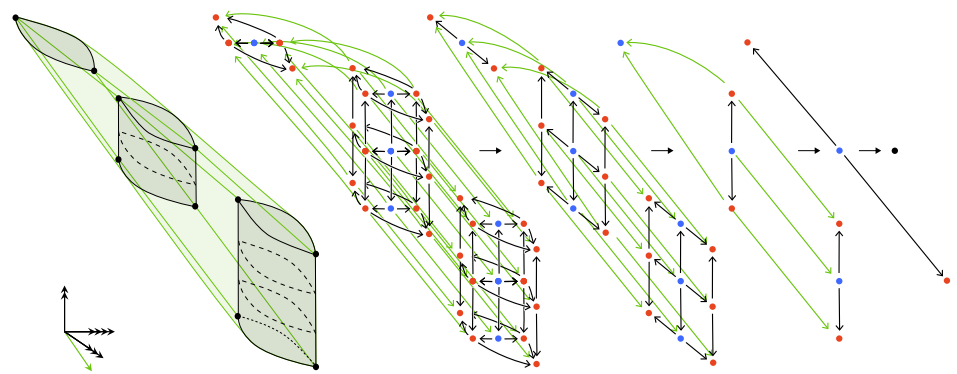
FIGURE B.9. Product of the 2-simplex and the 2-globe as a framed 4-cell.
