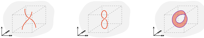
FIGURE 5.5. 3-Tame embeddings.
