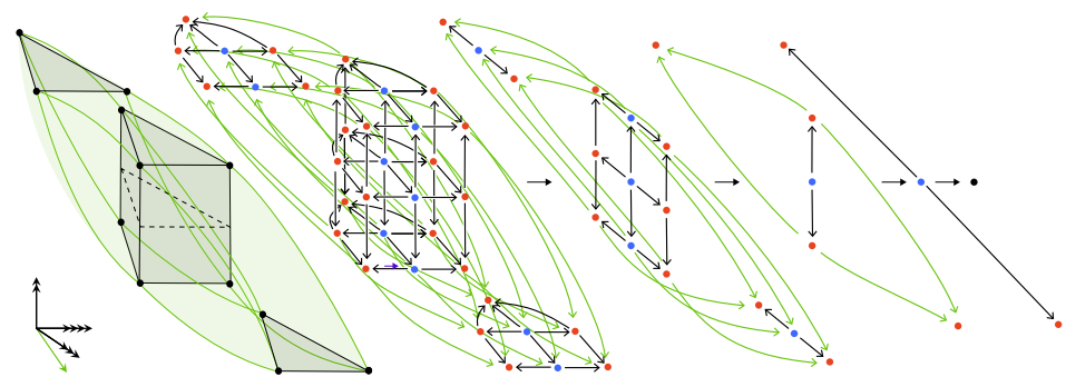
FIGURE B.10. Product of the 2-globe and the 2-simplex as a framed 4-cell.
