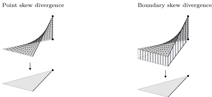
FIGURE 4.11. Subtle skews of mesh lift uniqueness.
