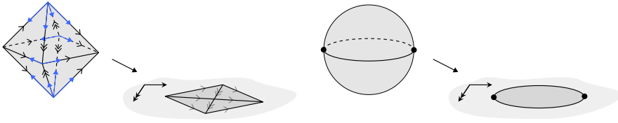
FIGURE 1.42. A 2-framed cell complex with a framed realization.
