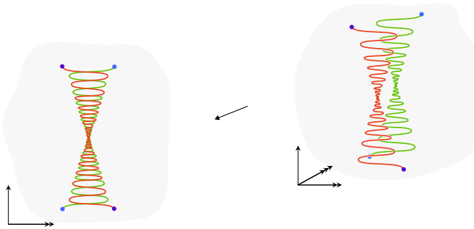
FIGURE 5.7. Nonlocal untameness.
