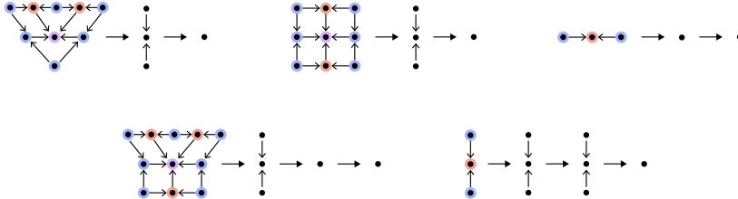
FIGURE 5.27. Truss singularities.
