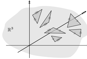
FIGURE 1.11. Framed realization of the 3-embedded framed 2-simplices.
