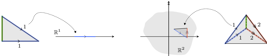
FIGURE 1.8. Framed realization of partially framed simplices.
