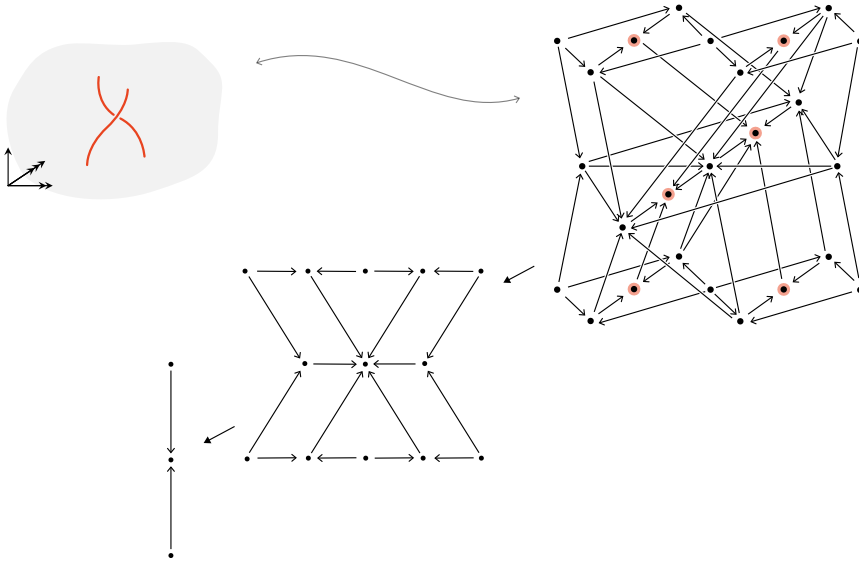
FIGURE 5.35. The normalized ambient stratified truss of the braid.
