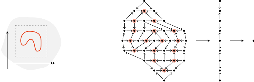
FIGURE 5.32. The normalized ambient stratified truss of the bean.
