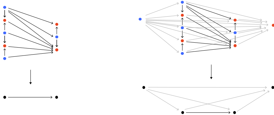
FIGURE 2.25. A 1-truss bundle and its suspension bundle.
