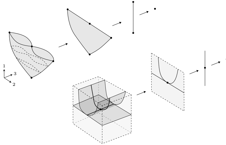
FIGURE I.10. A mesh block and its dual mesh brace.
