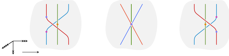
FIGURE 5.48. A manifold 3-diagram isotopy.
