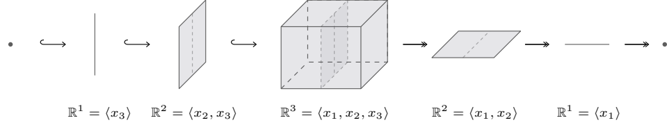
FIGURE A.2. The standard indframe and proframe.
