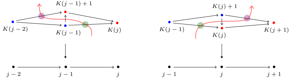
FIGURE 2.32. The construction of successor sections.
