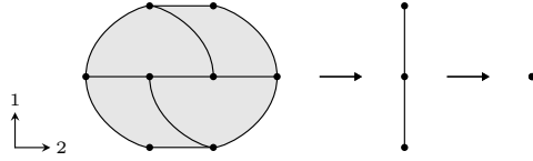
FIGURE I.6. A closed 2-mesh.
