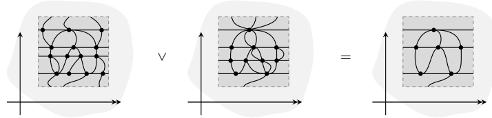
FIGURE 5.13. The join of two open 2-meshes.
