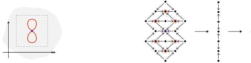
FIGURE 5.33. The normalized ambient stratified truss of the figure-8.
