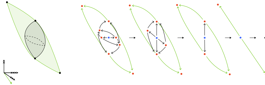
FIGURE B.7. The 4-globe as a framed 4-cell.
