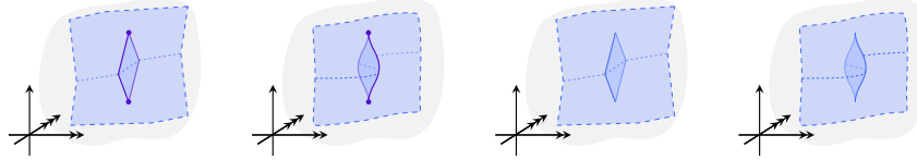
FIGURE 5.45. Framed conical and not framed conical embeddings.
