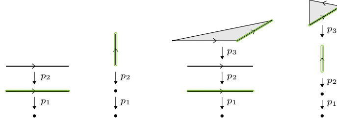
FIGURE 3.8. Embedded profamed simplices.
