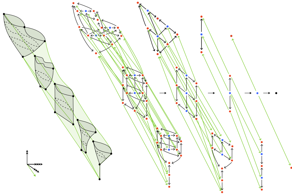
FIGURE B.11. A more involved framed 4-cell.
