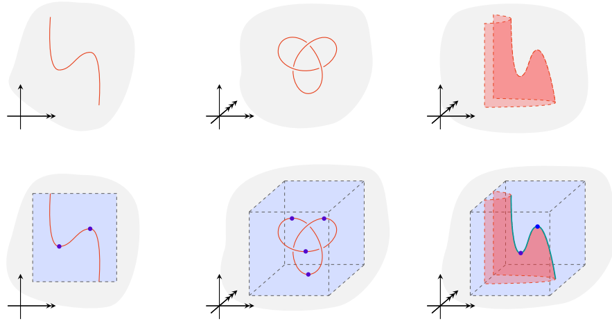
FIGURE 5.49. Tame tangles and their refining manifold diagrams.
