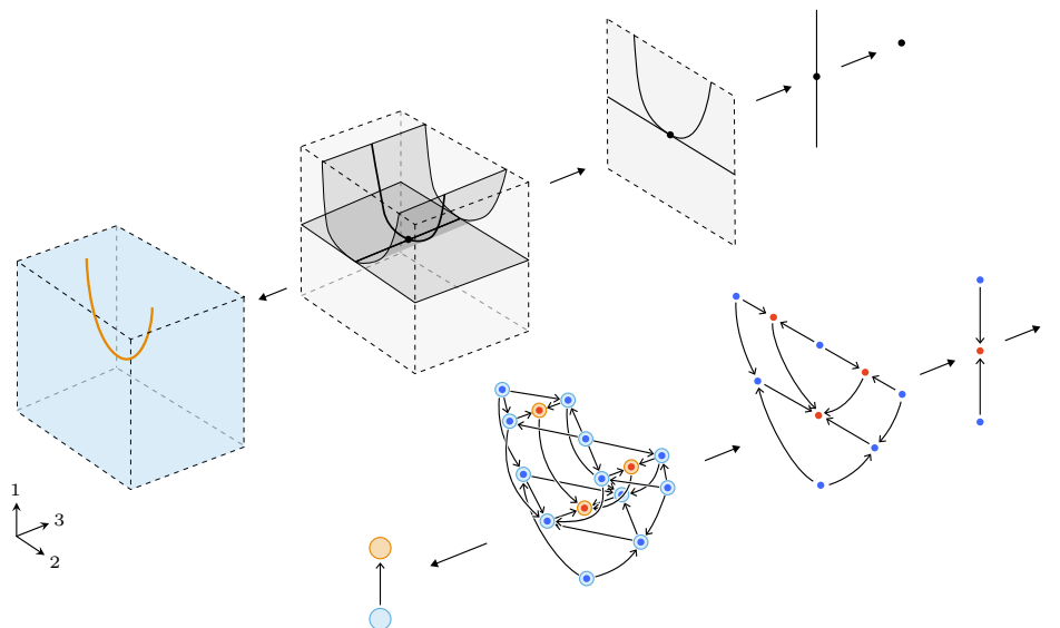
FIGURE I.16. A tame stratification, its coarsest mesh, and its normalized stratified truss.
