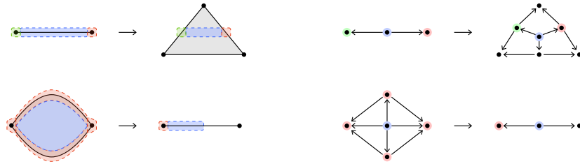
FIGURE 1.38. Non-cellular maps of regular cells.
