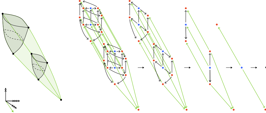
FIGURE B.8. The double cone of the 2-globe as a framed 4-cell.
