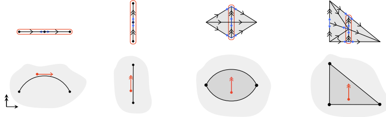
FIGURE 1.56. Highest frame vectors and axel vectors of framed 1-cells and 2-cells.
