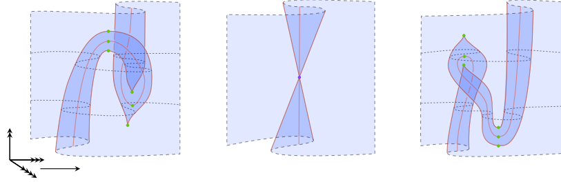
FIGURE 5.47. A manifold 4-diagram.
