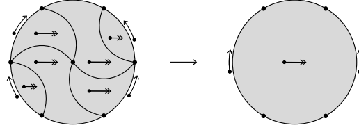
FIGURE I.8. A framed cell subdivision.
