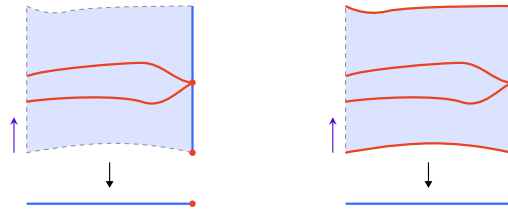
FIGURE 4.13. The compactification of a 1-mesh bundle.
