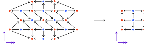
FIGURE I.9. A truss block subdivision.
