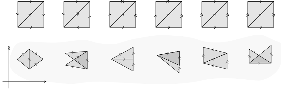
FIGURE 1.24. Simplicial complexes with 2-framings and their framed realizations.
