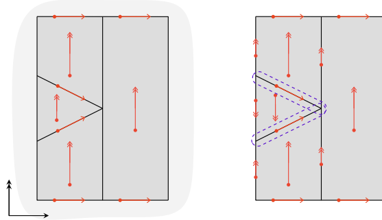
FIGURE 1.44. Collapsible and non-collapsible 2-framed cell complexes.
