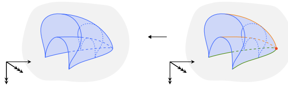
FIGURE 5.51. A projection of a 3-tangle singularity and its critical refinement.
