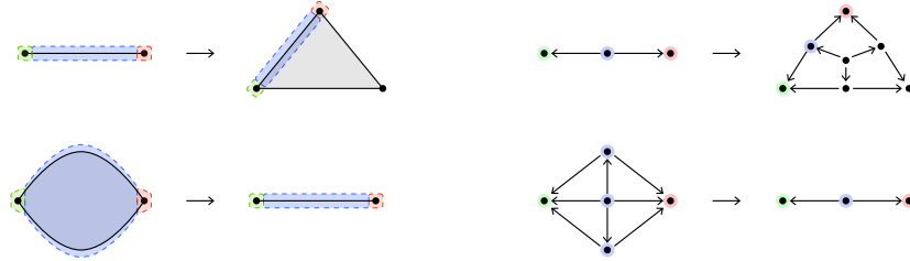
FIGURE 1.37. Cellular maps of regular cells.
