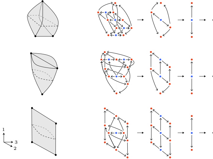
FIGURE I.5. Framed 3-cells and their truss blocks.
