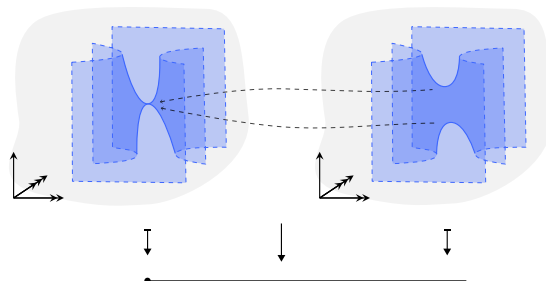
FIGURE 5.53. A perturbation of the monkey saddle into two ordinary saddle singularities.
