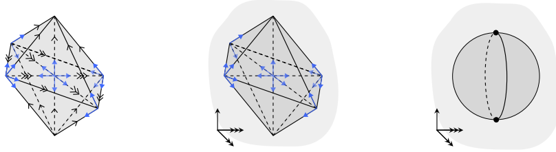
FIGURE 1.49. The simplest framed 3-cell.
