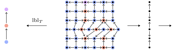
FIGURE 5.24. A stratified 2-truss represented by a poset labeling.
