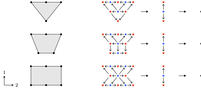
FIGURE I.4. Framed 2-cells and their truss blocks.
