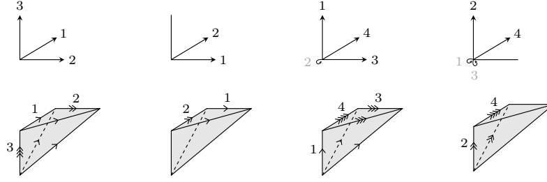
FIGURE 1.3. Frames, partial frames, embedded frames, and embedded partial frames on vector spaces and on simplices.
