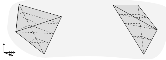
FIGURE 1.52. Realizations of regular 3-cells that are not framed regular cells.
