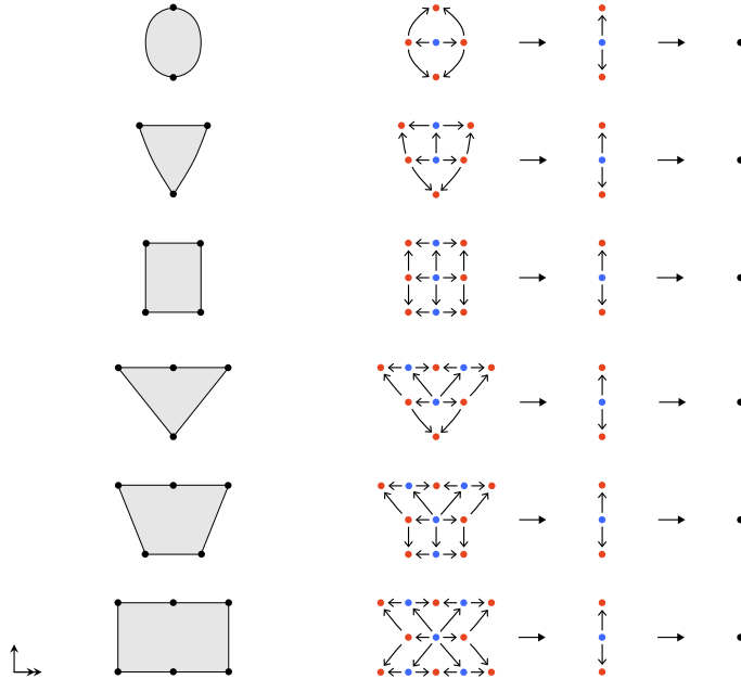
FIGURE B.1. Framed 2-cells.
