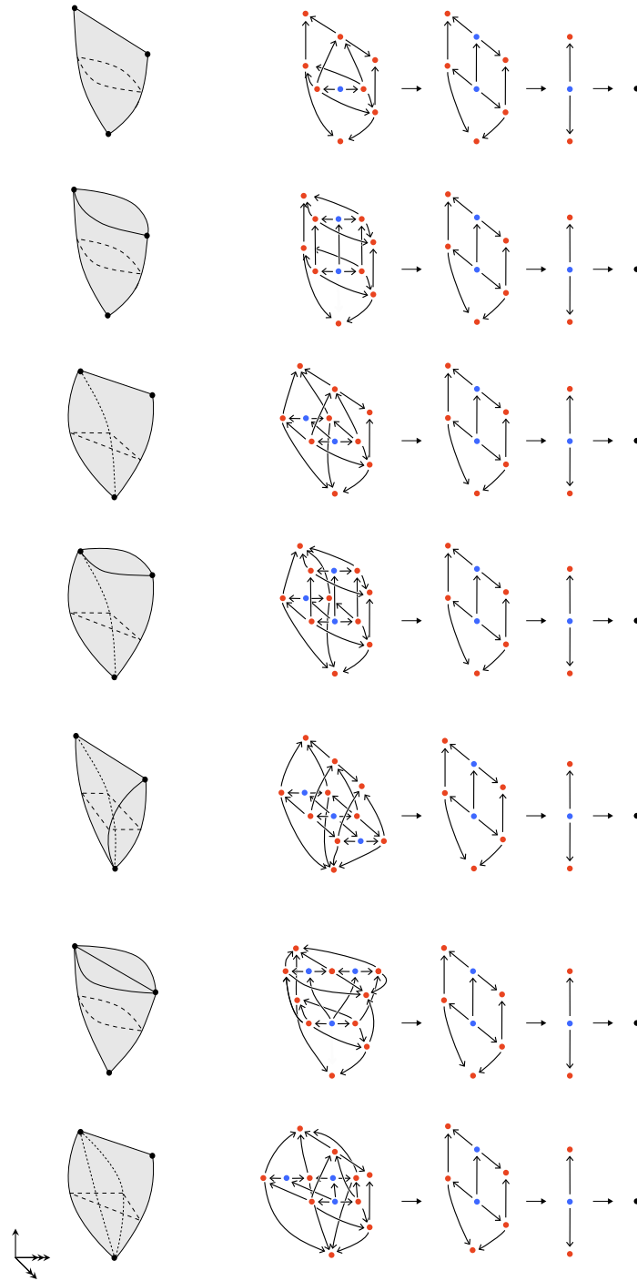
FIGURE B.3. Framed 3-cells projecting to the 2-simplex.
