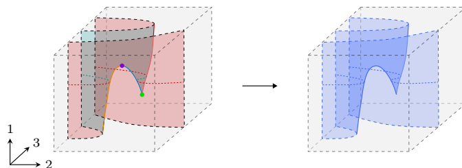
FIGURE 5.43. A manifold diagram and a tame tangle.
