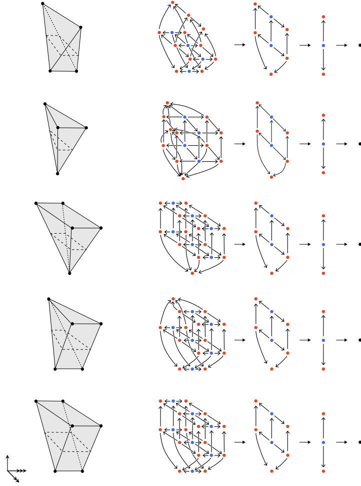
FIGURE B.4. Further framed 3-cells projecting to the 2-simplex.
