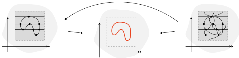
FIGURE 5.17. Refining meshes of a tame embedding.
