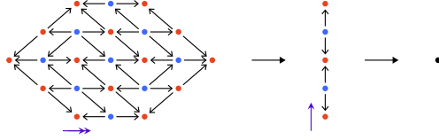
FIGURE I.2. A closed 2-truss.
