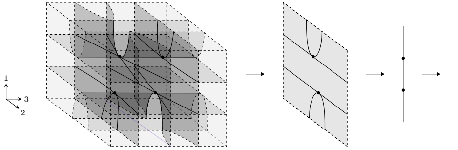
FIGURE I.7. An open 3-mesh.
