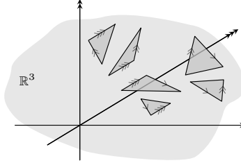
FIGURE 1.11. Framed realization of the 3-embedded framed 2-simplices.
