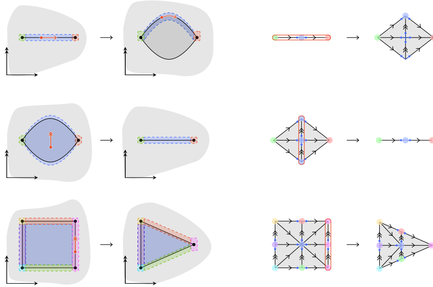
FIGURE 1.58. Framed cellular maps.
