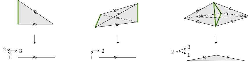
FIGURE 1.12. Embedded partially framed simplices.
