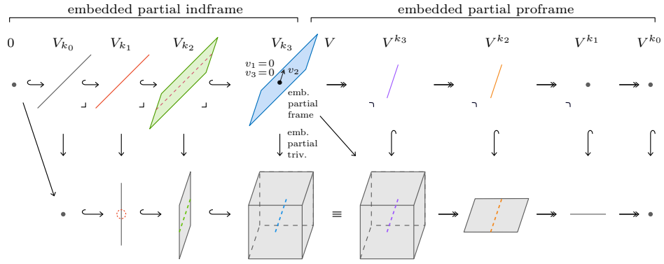
FIGURE A.6. 3-Embedded 1-partial trivialization, frame, indframe, and proframe.
