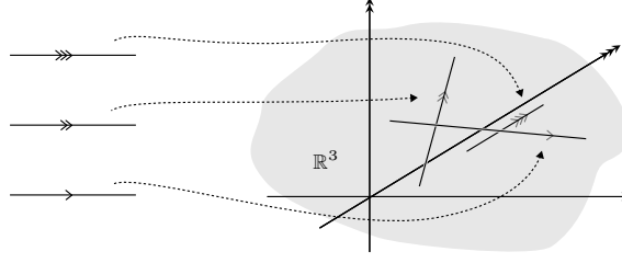
FIGURE 1.10. Framed realization of the 3-embedded framed 1-simplices.
