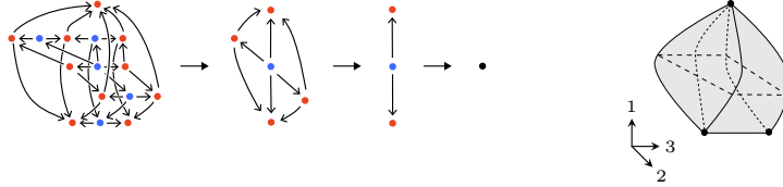
FIGURE 2.52. A 3-truss 3-block and its corresponding framed 3-cell.
