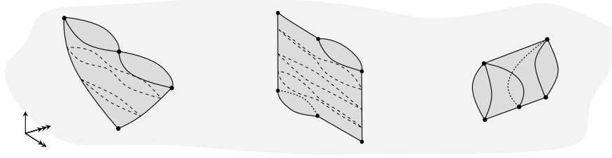
FIGURE 1.54. Yet more framed 3-cells.
