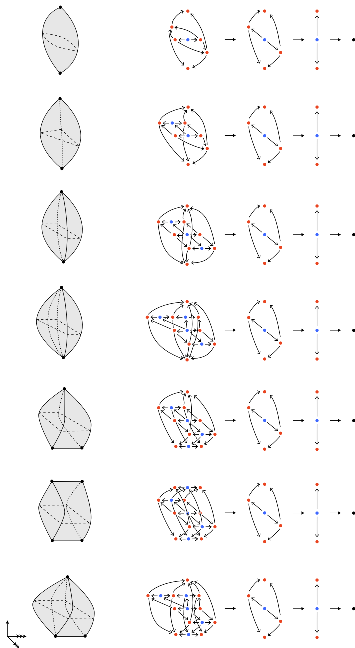
FIGURE B.2. Framed 3-cells projecting to the 2-globe.
