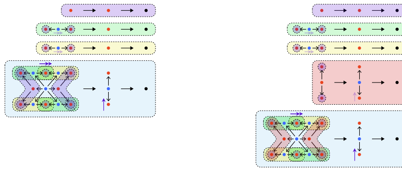
FIGURE 2.54. The blocks of a block set and of a block complex.
