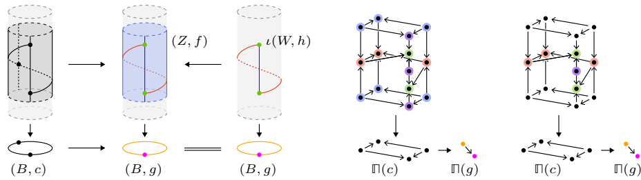
FIGURE 5.36. A tame stratified bundle and a tame bundle embedding with corresponding normalized stratified truss bundles.
