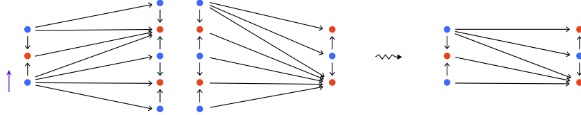
FIGURE 2.16. Composition of 1-truss bordisms.
