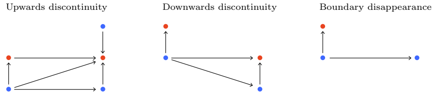
FIGURE 2.13. Fixable failures of truss bifunctionality.
