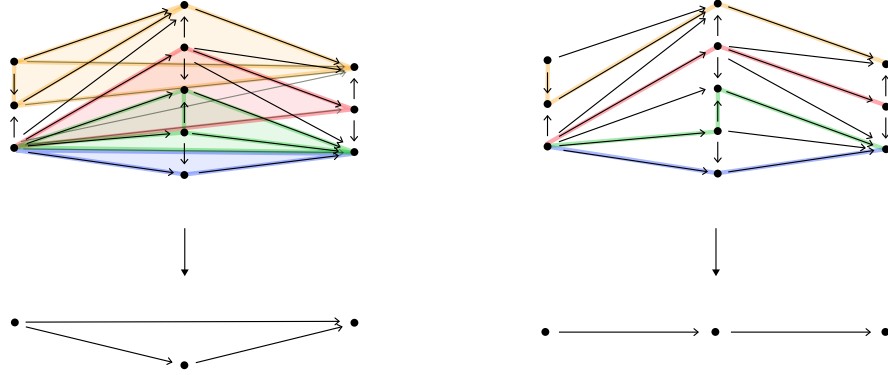
FIGURE 2.28. Spine notation for sections and spacers.
