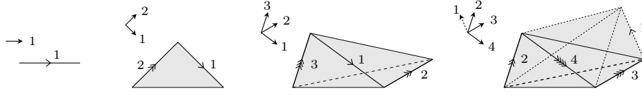
FIGURE 1.4. Framed simplices.
