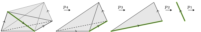
FIGURE 3.6. A proframed 4-simplex.
