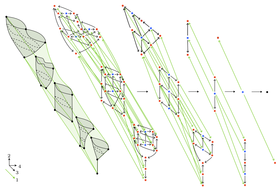
FIGURE C.11. A more involved 4-cell.
