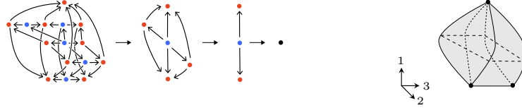
FIGURE 2.52. A 3-truss 3-block and its corresponding framed 3-cell.
