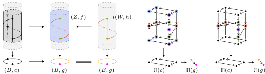
FIGURE 5.35. A tame stratified bundle and a tame bundle embedding with corresponding normalized stratified truss bundles.
