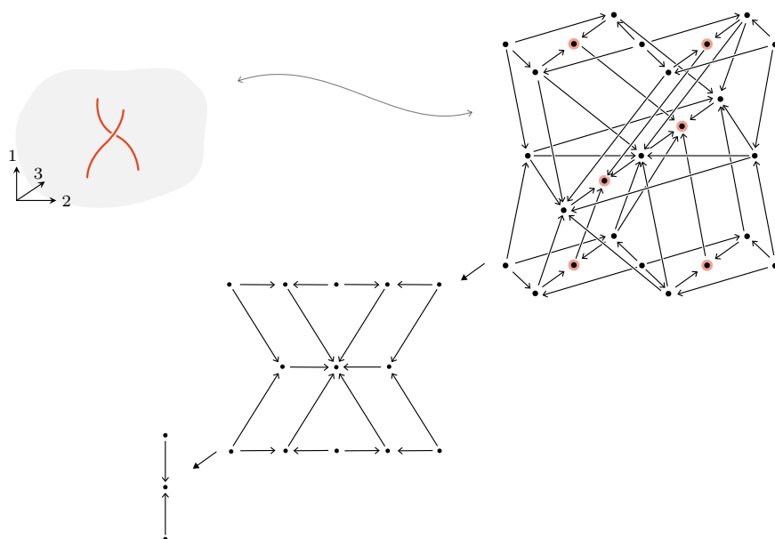
FIGURE 5.34. The normalized ambient stratified truss of the braid.
