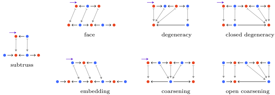
FIGURE 2.48. Faces, embeddings, degeneracies, and coarsenings.
