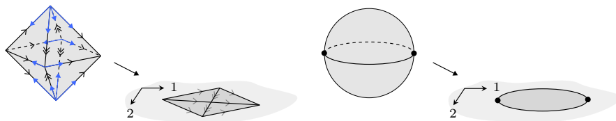
FIGURE 1.42. A 2-framed regular cell complex with a framed realization.
