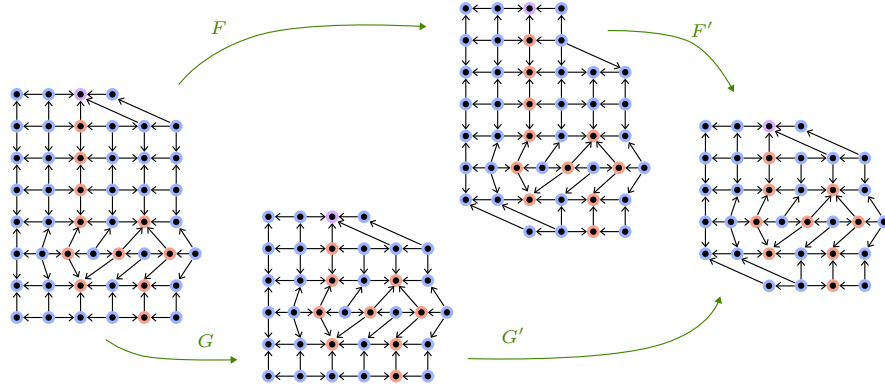
FIGURE 5.37. Confluence of truss coarsenings.
