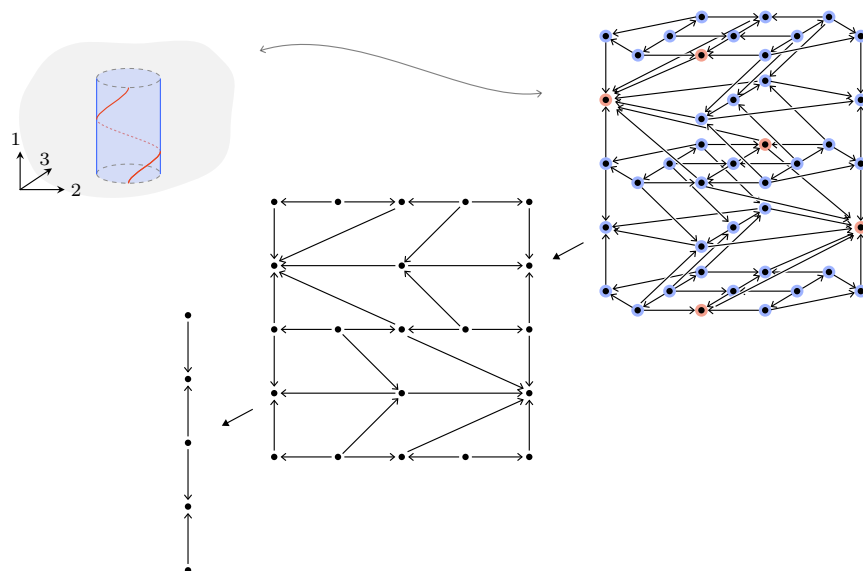
FIGURE 5.33. The normalized stratified truss of a 3-tame stratification.
