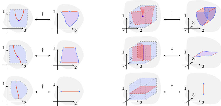
FIGURE 5.38. Tame singularities and their dual tame cells.
