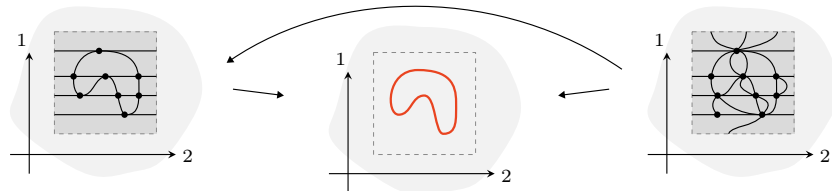
FIGURE 5.17. Refining meshes of a tame embedding.
