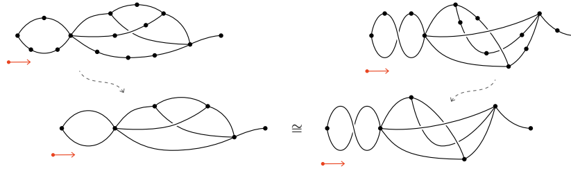
FIGURE 5.42. Decidability of framed homeomorphism for 1-DAGs.
