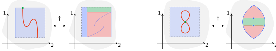
FIGURE 5.39. Duality of tame stratifications.
