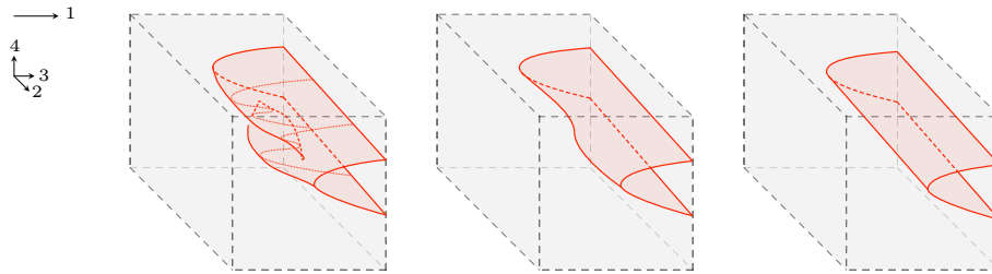
FIGURE I.9. A tame stratification with a swallowtail singularity.
