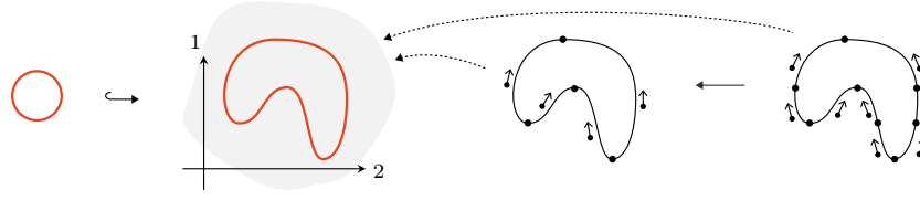
FIGURE 5.41. Coarsest cell structure of a tamely embedded circle.
