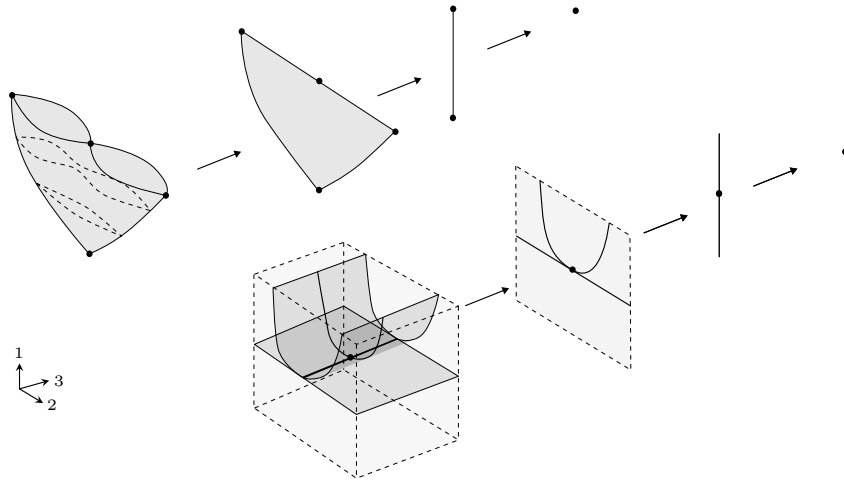
FIGURE I.7. A mesh block and its dual mesh brace.
