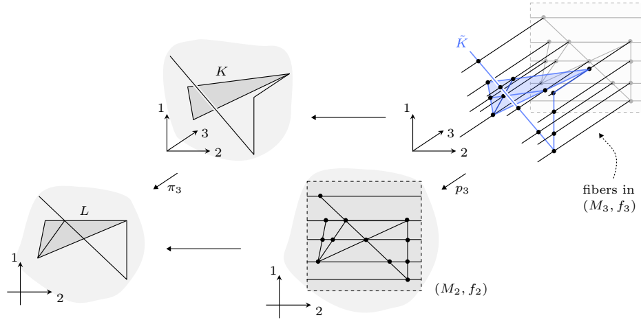
FIGURE 5.36. Inductive construction of mesh refinements for polyhedral stratifications.
