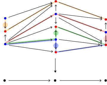
FIGURE 2.30. Spacers and their associated fiber morphisms.
