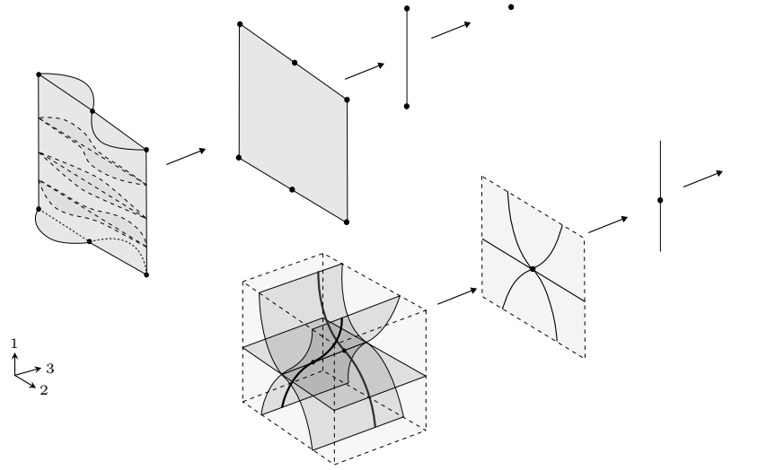
FIGURE I.8. A closed mesh and its dual open mesh.
