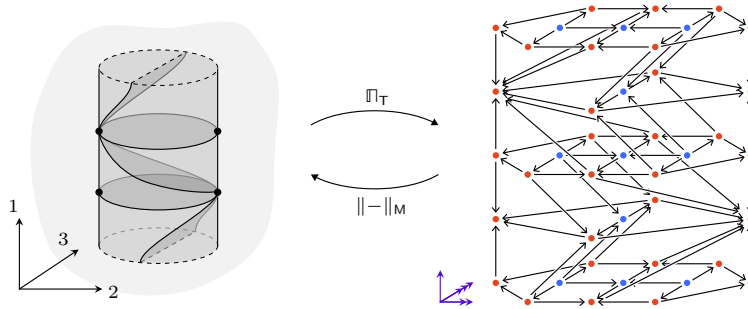
FIGURE 4.17. A corresponding 3-mesh and 3-truss.
