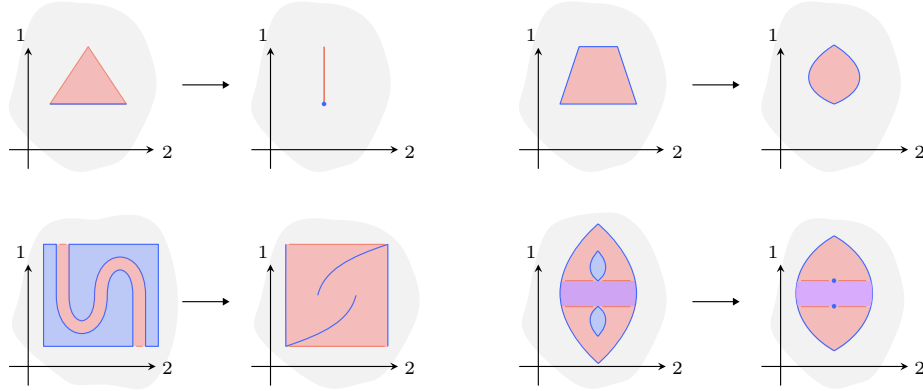
FIGURE 5.40. Degeneracies of tame stratifications.
