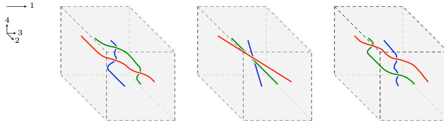
FIGURE I.10. A tame stratification with a Reidemeister III move.
