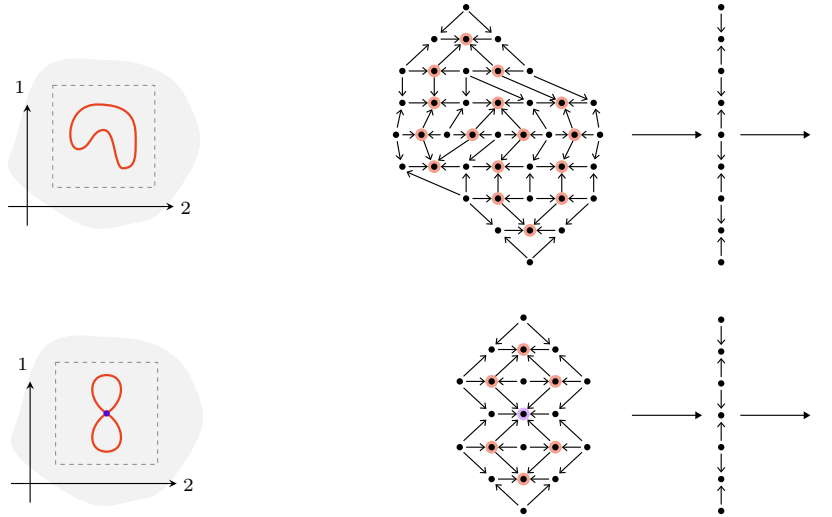
FIGURE 5.32. Normalized ambient stratified trusses classifying 2-tame embeddings.
