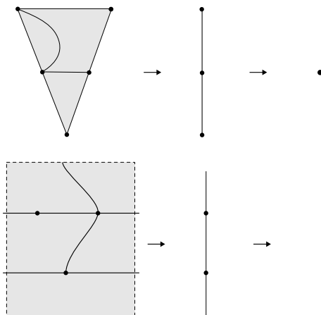
FIGURE 4.27. A closed mesh and its dual open mesh.
