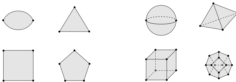
FIGURE 1.34. Regular 2-cells and regular 3-cells.
