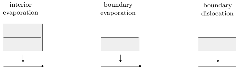
FIGURE 4.9. Lamentable lapses of liftability.
