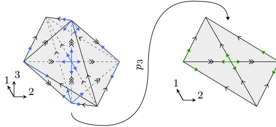
FIGURE 3.17. The projected 2-framed cell of a 3-framed cell.
