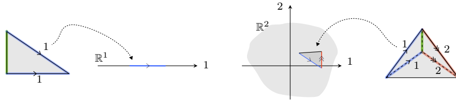
FIGURE 1.8. Framed realization of partially framed simplices.
