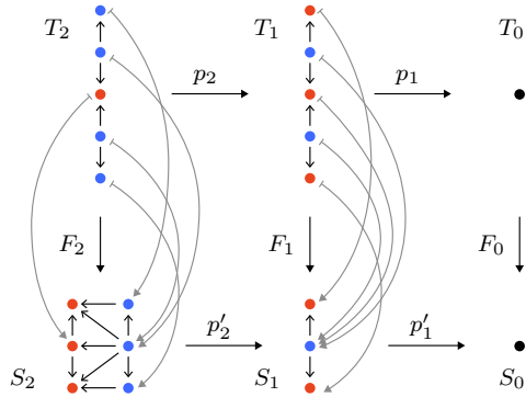
FIGURE 2.50. Failure of epi-mono factorization of a 2-truss map.
