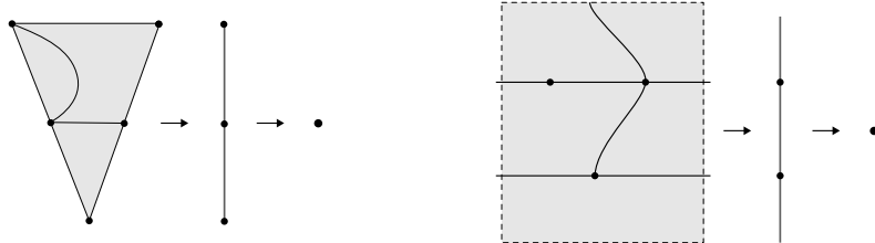
FIGURE 4.27. A closed mesh and its dual open mesh.
