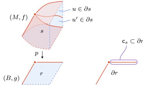
FIGURE 4.19. The regular contour of a regular stratum.
