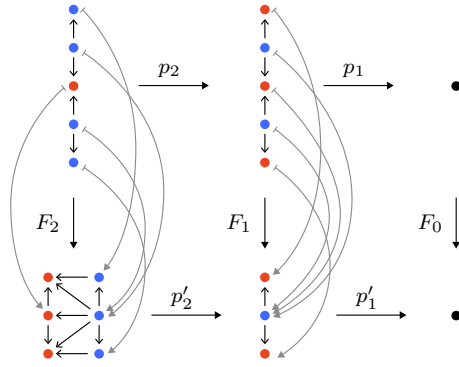
FIGURE 2.50. Failure of epi-mono factorization of a 2-truss map.
