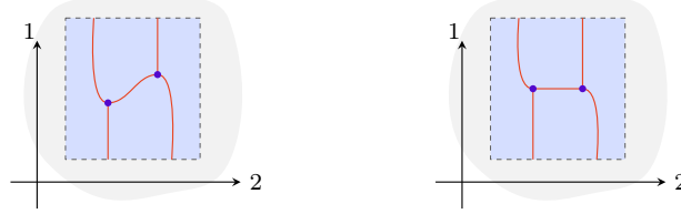
FIGURE 5.47. A manifold diagram and not a manifold diagram.
