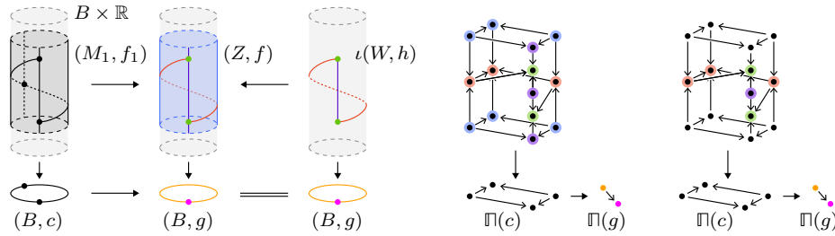
FIGURE 5.35. A tame stratified bundle and a tame bundle embedding with corresponding normalized stratified truss bundles.
