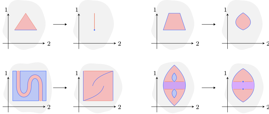
FIGURE 5.40. Degeneracies of tame stratifications.
