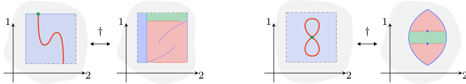
FIGURE 5.39. Duality of tame stratifications.
