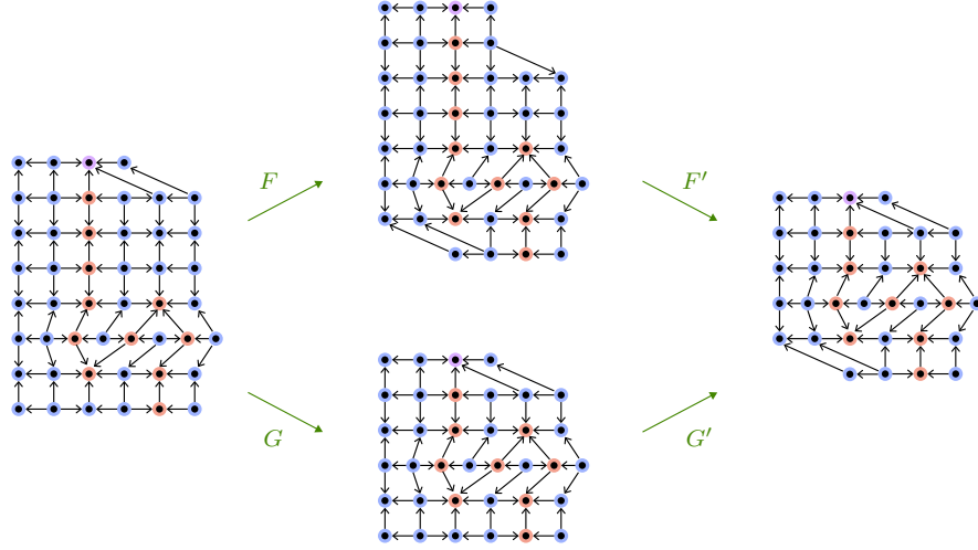
FIGURE 5.37. Confluence of truss coarsenings.
