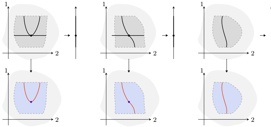
FIGURE 5.29. Mesh singularities.
