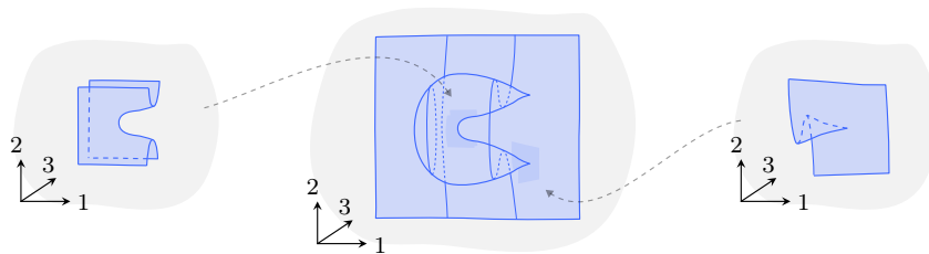
FIGURE 5.50. Two tangle singularities in a tame 2-tangle.
