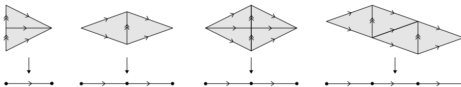
FIGURE 1.28. Collapsible 2-framed simplicial complexes with their 2-collapse maps.
