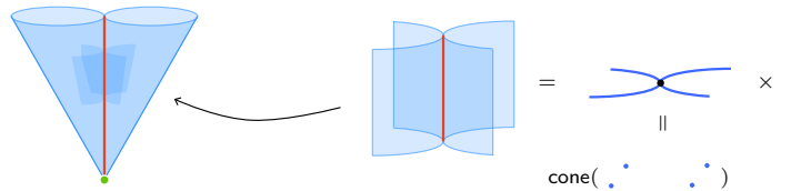
FIGURE B.13. A conical stratification with a tubular neighborhood.
