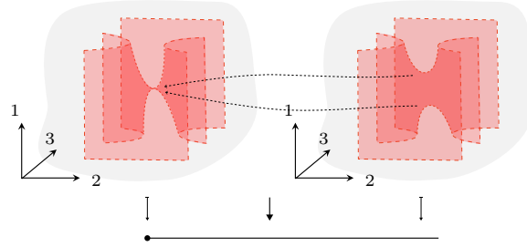
FIGURE 5.51. A perturbation of the monkey saddle into two ordinary saddle singularities.
