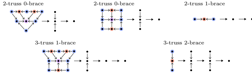
FIGURE 5.27. Truss singularities.
