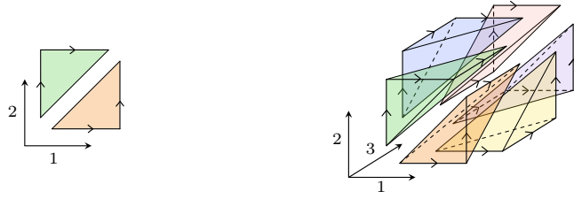
FIGURE 1.1. Distinct framed standard simplices spanned by the same standard frame vectors.
