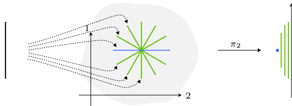
FIGURE 5.44. Genericity of framings on the embedded interval.
