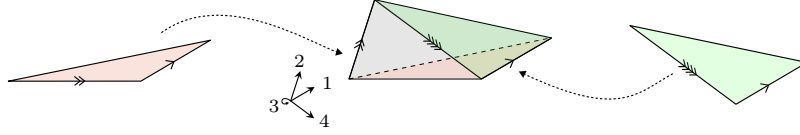
FIGURE 1.16. Restriction of an embedded frame to faces of a simplex.
