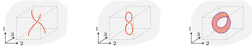
FIGURE 5.5. 3-Tame embeddings.
