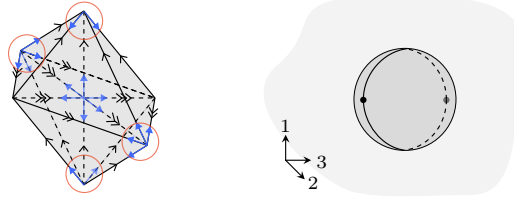
FIGURE 1.50. A framing of the simplicial complex underlying the regular 3-globe that does not yield a framed regular cell.
