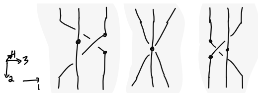
FIGURE 5.46. A manifold 3-diagram isotopy.
