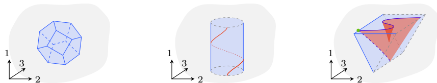
FIGURE 5.4. 3-Tame stratifications.
