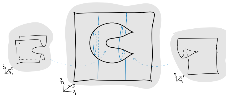
FIGURE 5.48. Two tangle singularities in a tame 2-tangle.
