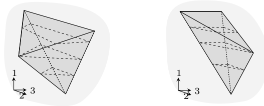
FIGURE 1.52. Realizations of 3-cells that are not framed regular cells.
