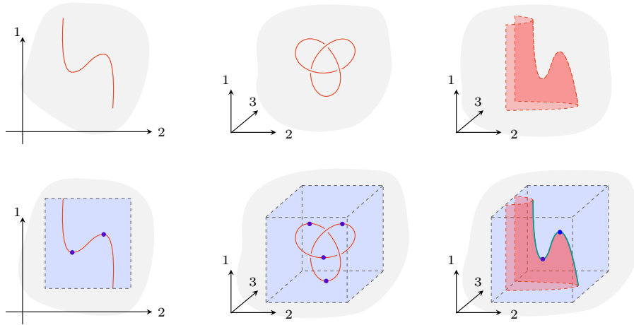
FIGURE 5.47. Tame tangles and their refining manifold diagrams.
