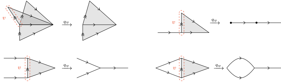
FIGURE 1.26. Elementary collapse of frame 2-vectors.
