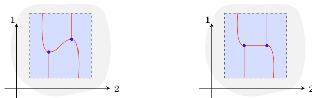
FIGURE 5.45. A manifold diagram and not a manifold diagram.
