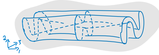
FIGURE 5.50. A 1-tangle isotopy.
