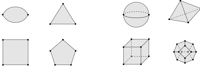
FIGURE 1.34. An illustration of regular 2-cells and 3-cells.
