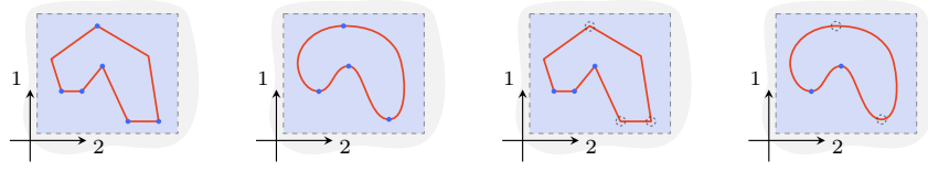
FIGURE 5.42. Framed conical and not framed conical stratifications.
