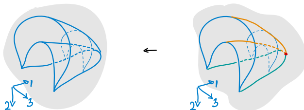
FIGURE 5.49. A projection of a 3-tangle singularity and its critical refinement.
