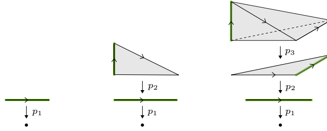
FIGURE 3.5. Proframed simplices.
