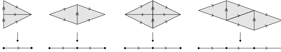
FIGURE 1.28. Collapsible 2-framed simplicial complexes with their 2-collapse maps.
