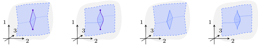
FIGURE 5.43. Framed conical and not framed conical embeddings.
