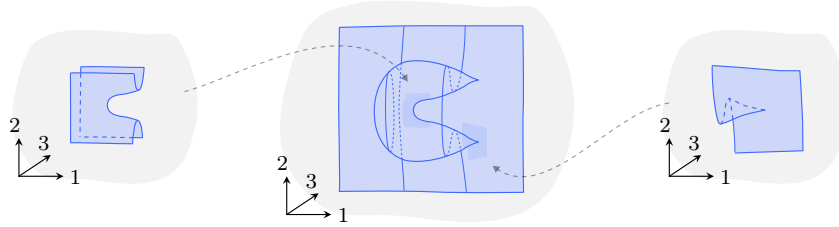
FIGURE 5.49. Two tangle singularities in a tame 2-tangle.
