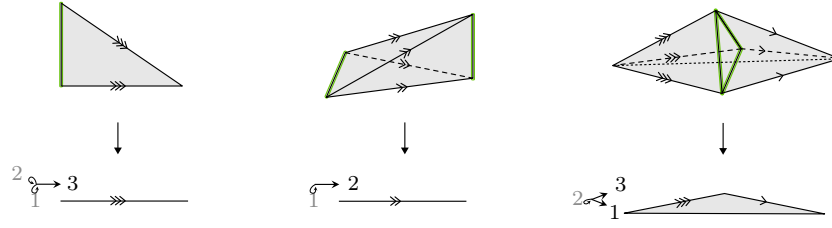
FIGURE 1.12. Embedded partially framed simplices.
