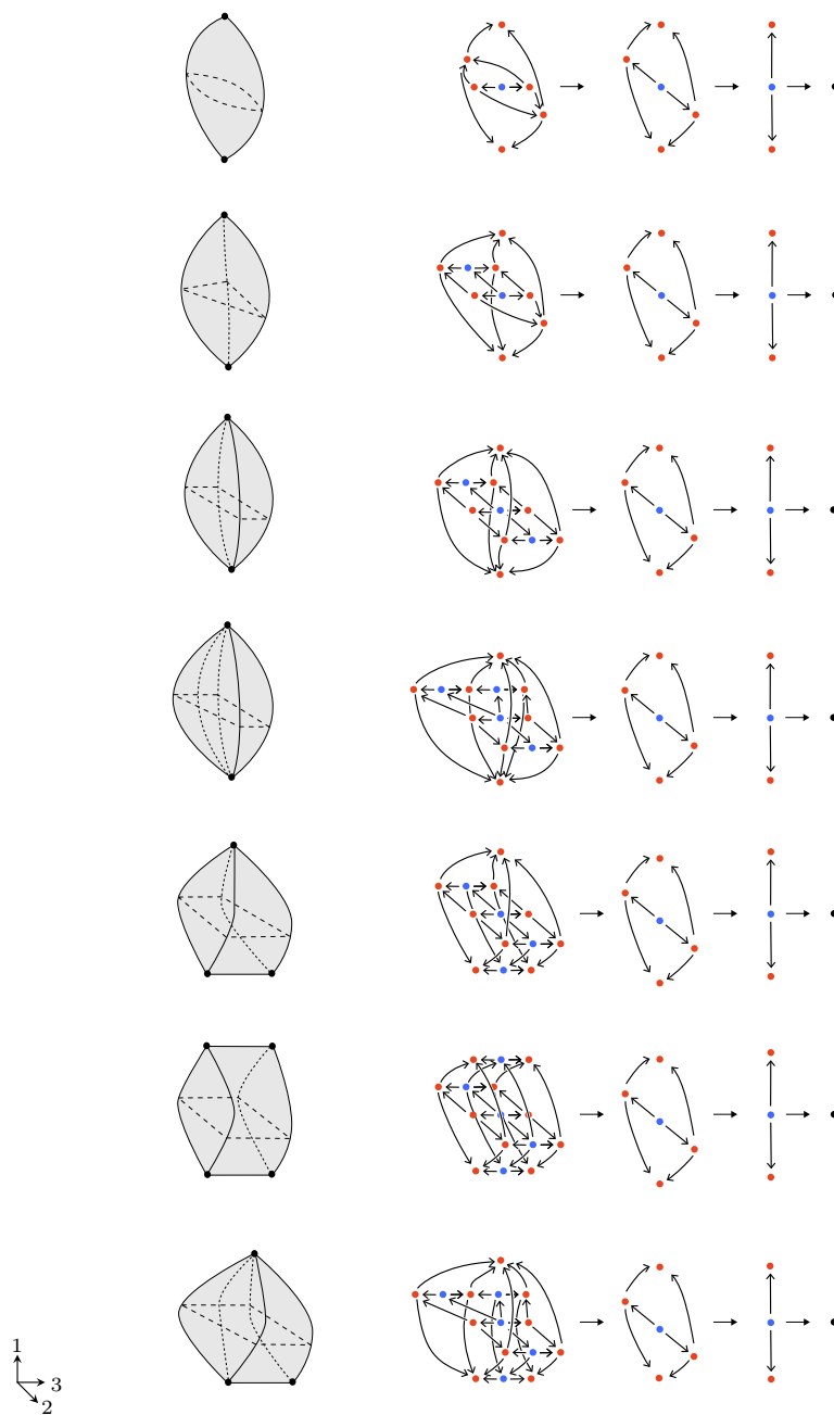
FIGURE B.2. Framed regular 3-cells projecting to the 2-globe.
