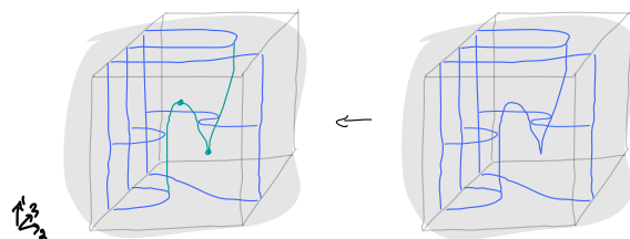
FIGURE 5.42. A manifold diagram and a tame tangle.
