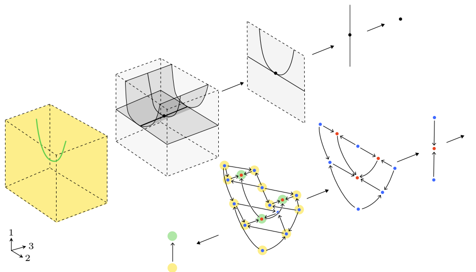
FIGURE I.13. A tame stratification, its coarsest mesh, and its normalized stratified truss.
