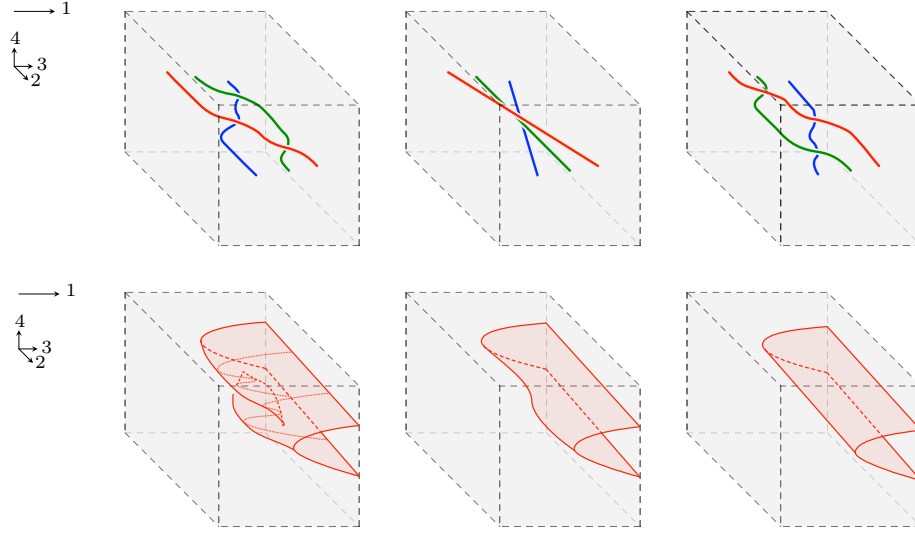
FIGURE I.10. A tame stratification with a Reidemeister III move.
