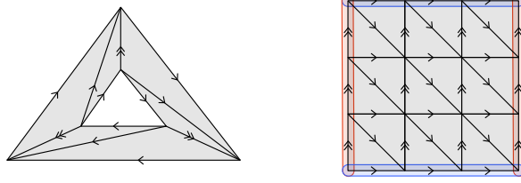
FIGURE 1.31. Progressive framed simplicial manifolds.
