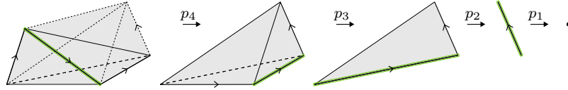
FIGURE 3.6. A proframed 4-simplex.
