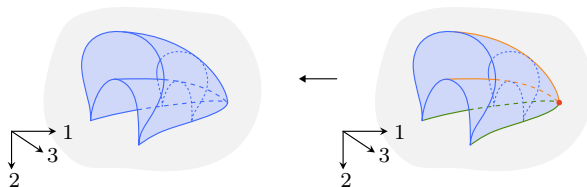
FIGURE 5.50. A projection of a 3-tangle singularity and its critical refinement.
