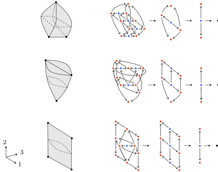
FIGURE I.4. Framed regular 3-cells and their truss blocks.
