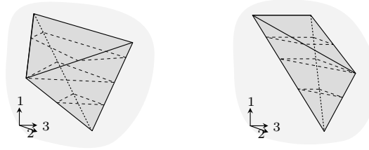
FIGURE 1.52. Realizations of regular 3-cells that are not framed regular cells.
