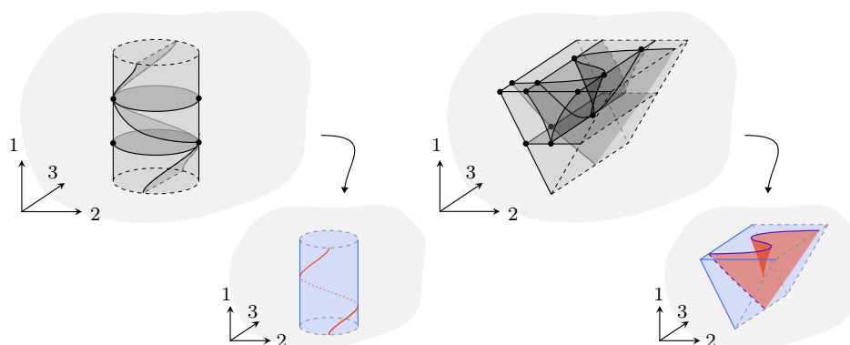
FIGURE 5.20. Coarsest meshes of 3-tame stratifications.
