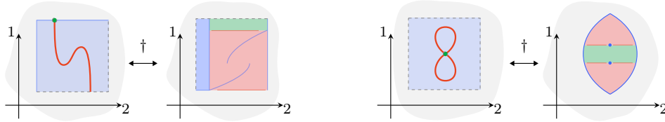
FIGURE 5.38. Duality of tame stratifications.
