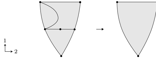
FIGURE I.6. A framed regular cell complex subdivision of a framed cell.
