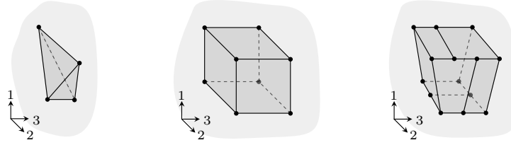
FIGURE 1.51. Simple framed regular 3-cells.
