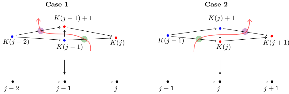
FIGURE 2.32. The construction of successor sections.
