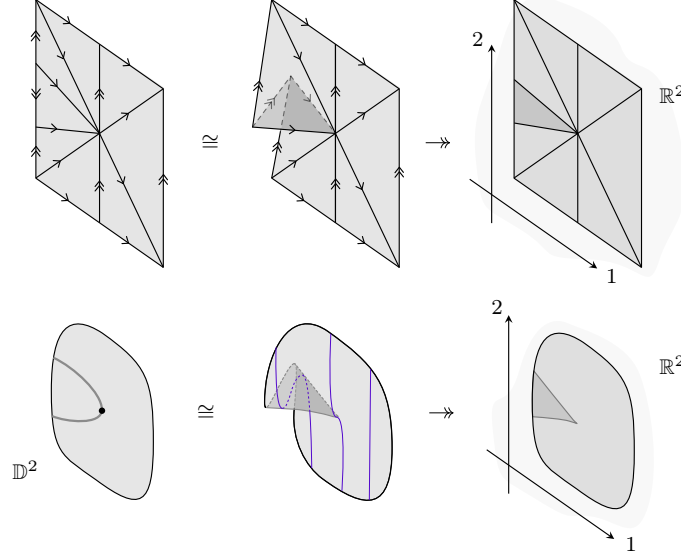
FIGURE 1.21. A framed simplicial complex and a differential singularity.
