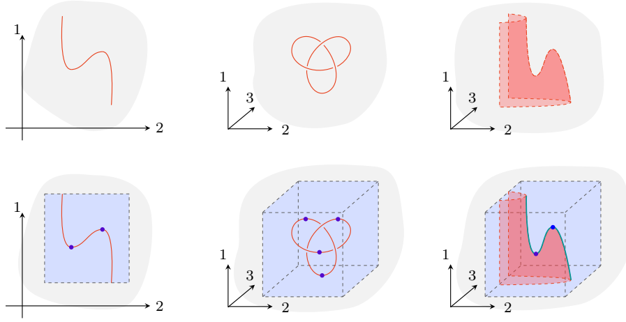
FIGURE 5.48. Tame tangles and their refining manifold diagrams.
