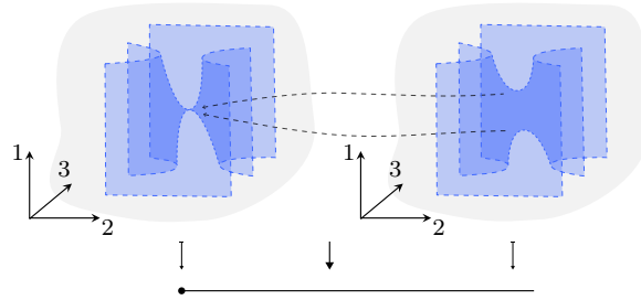
FIGURE 5.52. A perturbation of the monkey saddle into two ordinary saddle singularities.
