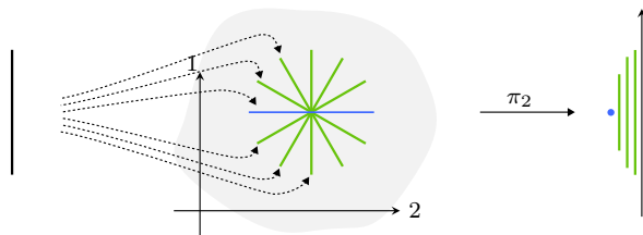
FIGURE 5.45. Genericity of framings on the embedded interval.
