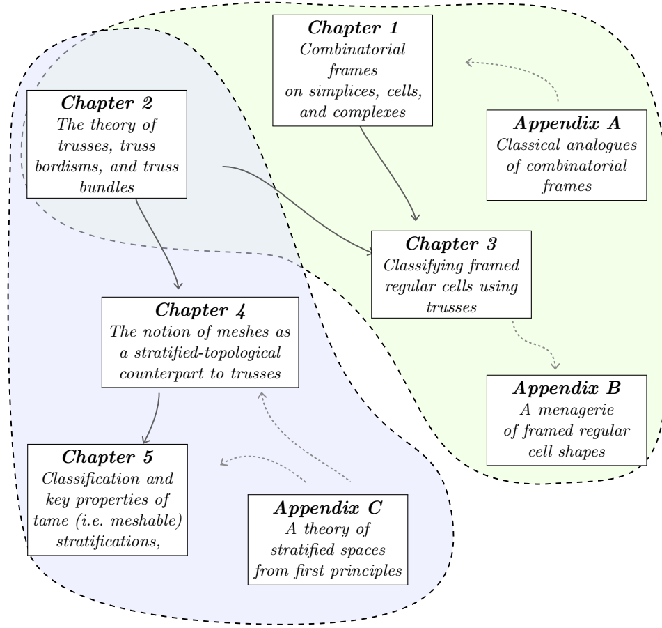
FIGURE I.15. Overview of dependencies.
