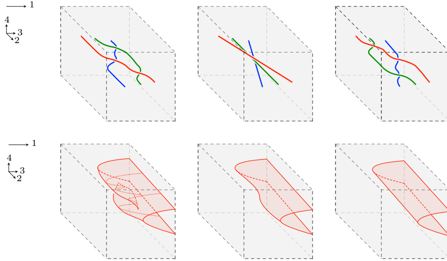
FIGURE I.9. A tame stratification with a swallowtail singularity.
