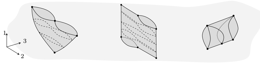
FIGURE 1.54. Yet more framed regular 3-cells.
