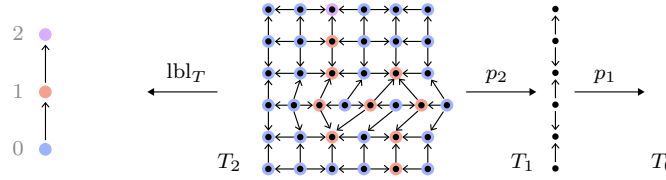
FIGURE 5.24. A stratified truss represented by a poset labeling.
