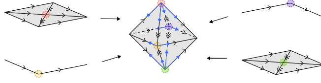
FIGURE 1.41. Collapsible subcomplexes of a 2-framed regular cell complex.
