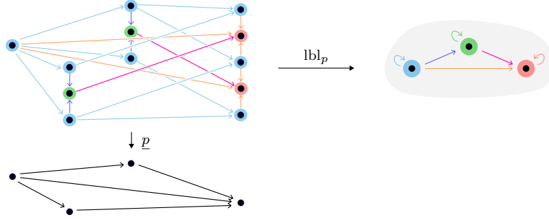
FIGURE 2.38. A 1-truss bundle labeled in a poset.
