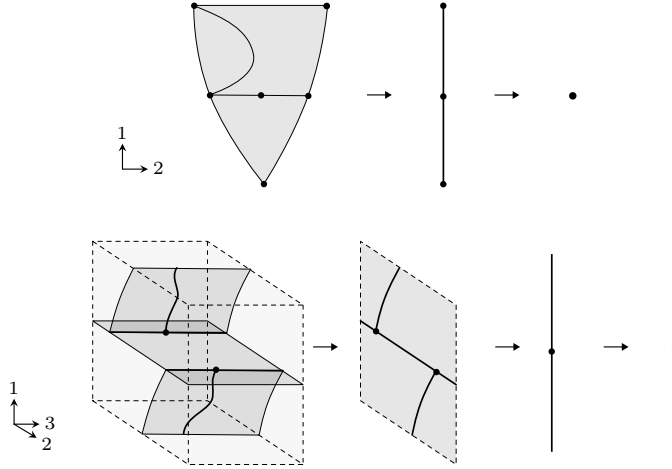
FIGURE I.5. A closed 2-mesh and an open 3-mesh.
