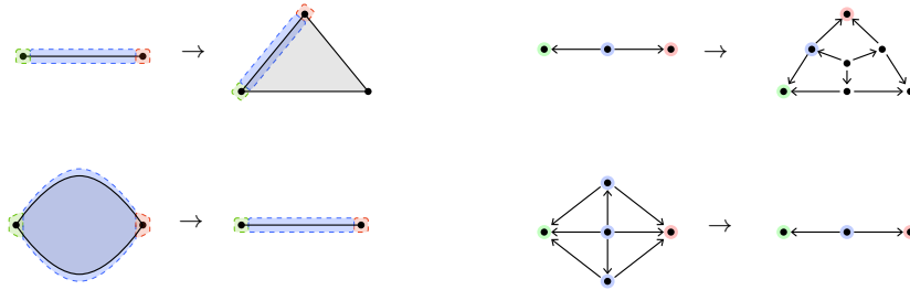
FIGURE 1.37. Cellular maps of regular cells.
