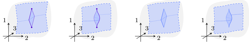
FIGURE 5.44. Framed conical and not framed conical embeddings.
