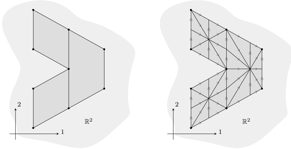
FIGURE 1.43. Framed realization of a framed regular cell complex.
