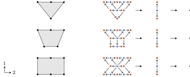
FIGURE I.3. Framed regular 2-cells and their truss blocks.
