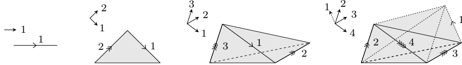
FIGURE 1.4. Framed simplices.
