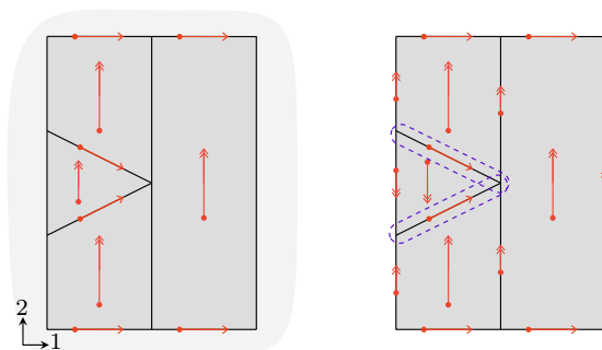
FIGURE 1.44. Collapsible and non-collapsible framed regular cell complexes.
