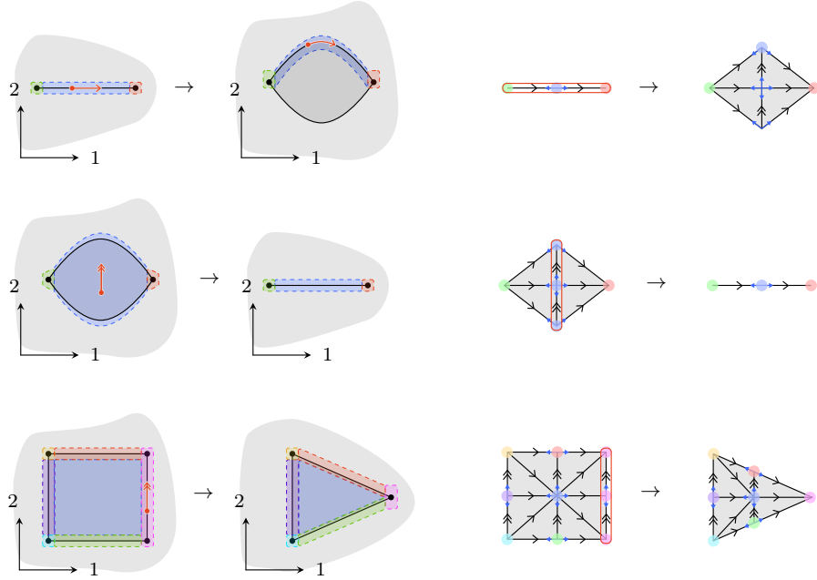
FIGURE 1.58. Framed cellular maps.
