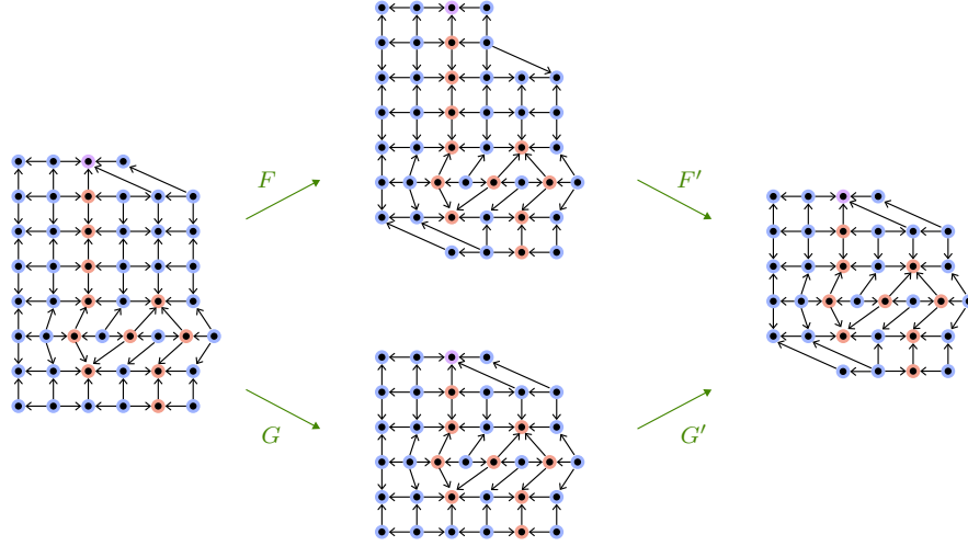
FIGURE 5.36. Confluence of truss coarsenings.
