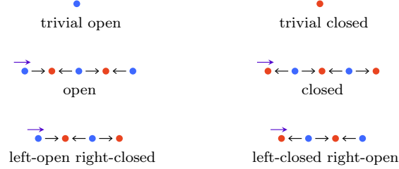
FIGURE 2.7. Endpoint types of 1-trusses.
