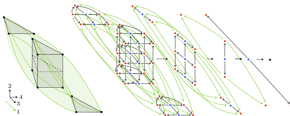
FIGURE B.10. The product of the 2-globe and the 2-simplex as a framed regular 4-cell.
