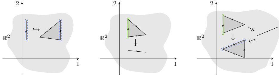
FIGURE 1.19. Framed maps via framed realization.
