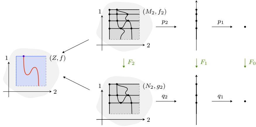
FIGURE 5.28. A mesh coarsening of stratified meshes.
