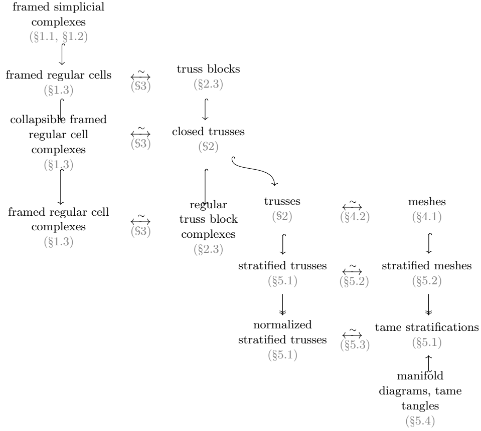
FIGURE I.14. Overview of concepts and connections.
