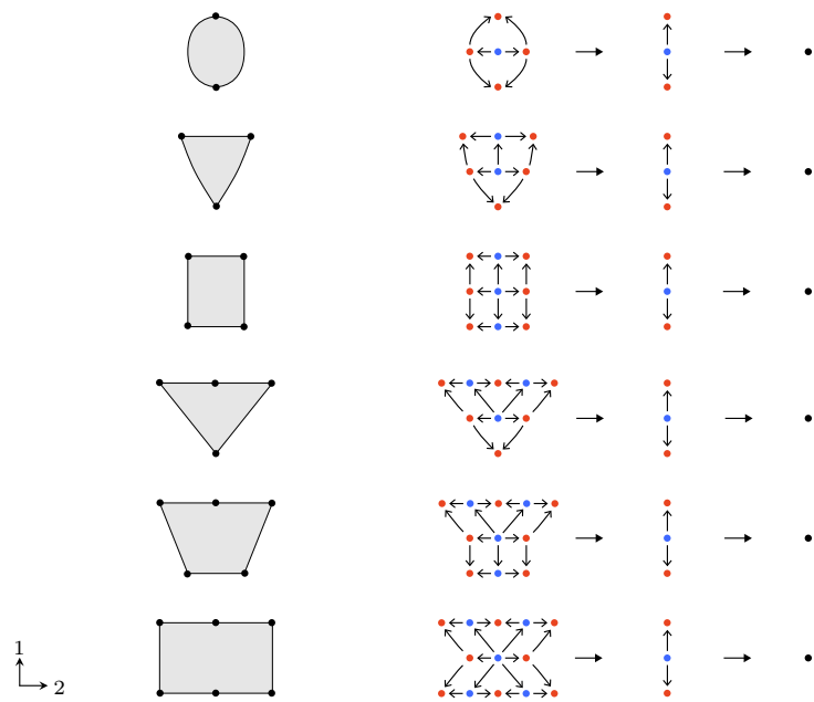
FIGURE B.1. Framed regular 2-cells.
