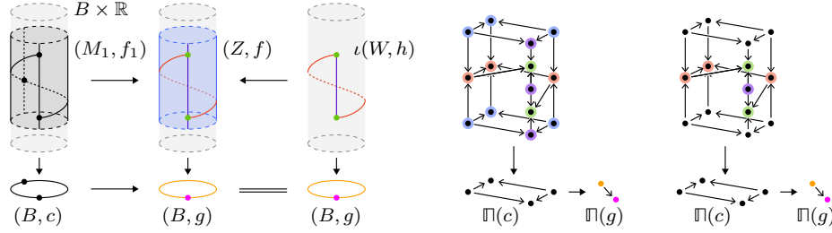
FIGURE 5.34. Tame stratified bundles and tame bundle embeddings with their corresponding normalized stratified truss bundles.
