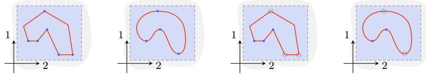
FIGURE 5.43. Framed conical and not framed conical stratifications.
