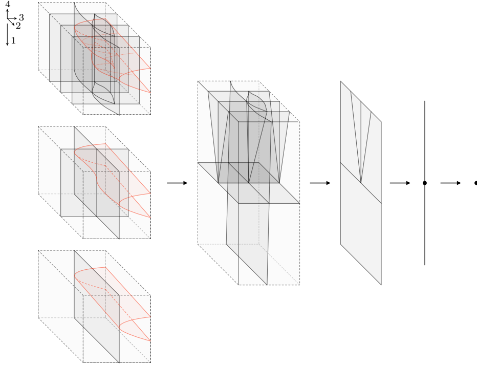
FIGURE I.11. The coarsest refining mesh of the swallowtail singularity.
