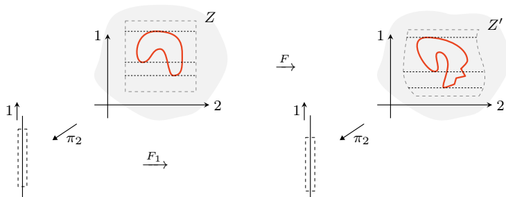
FIGURE 5.8. Framed stratified homeomorphism.
