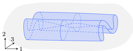
FIGURE 5.51. A 1-tangle isotopy.
