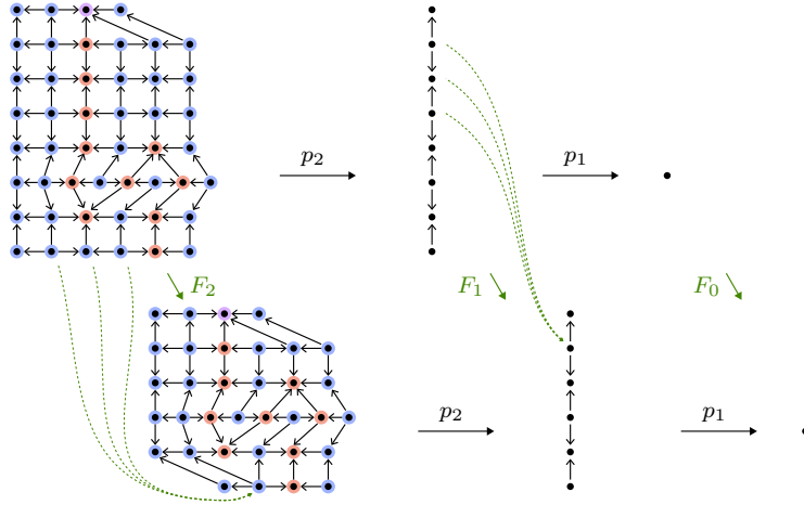
FIGURE 5.26. A truss coarsening of stratified trusses.
