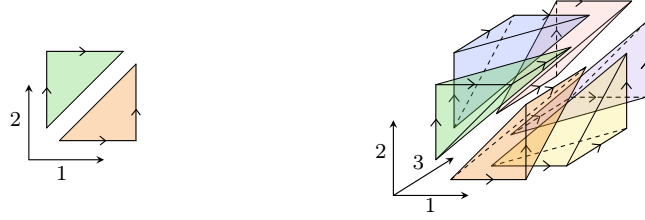
FIGURE 1.1. Distinct framed simplices spanned by the same standard frame vectors.
