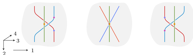
FIGURE 5.47. A manifold 3-diagram isotopy.
