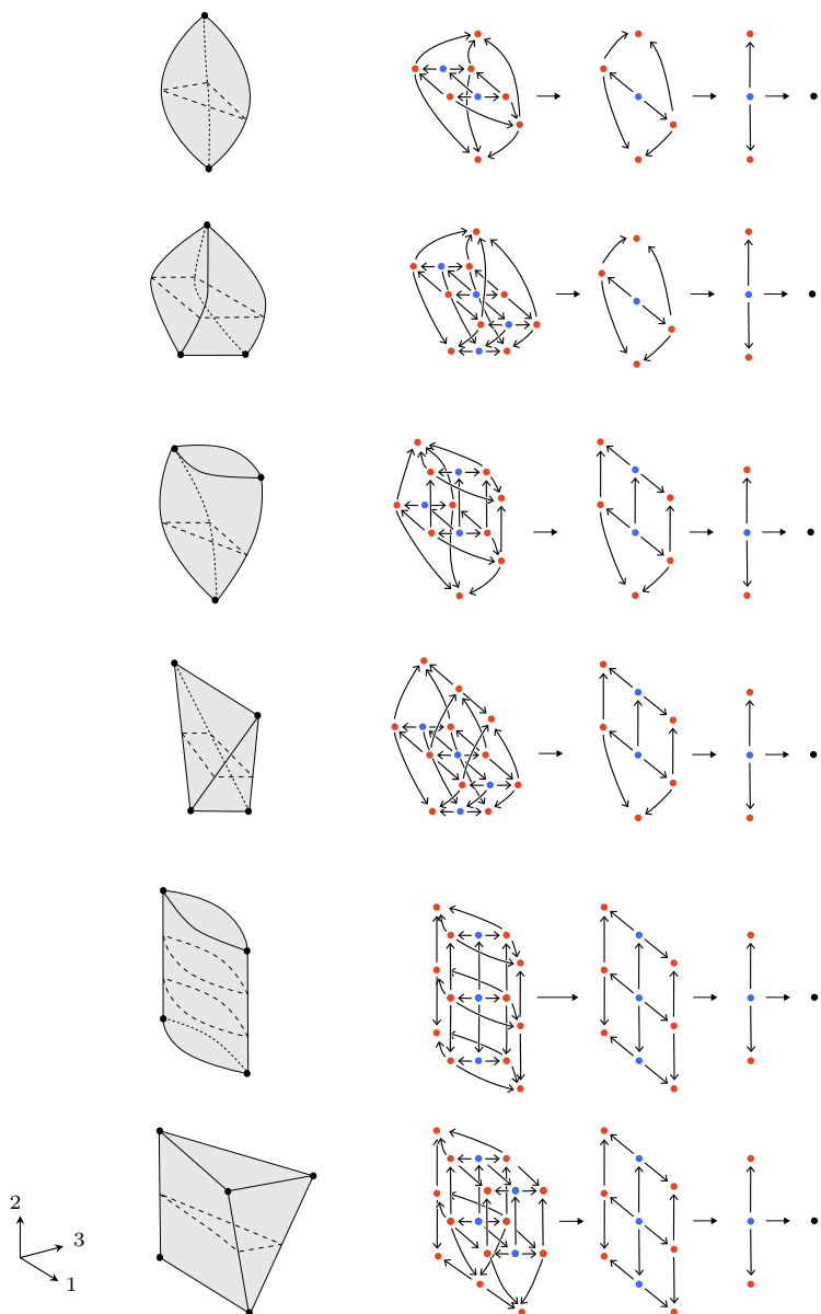
FIGURE I.3. Framed regular 3-cells and their classifying truss blocks.
