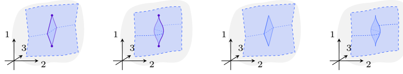
FIGURE 5.44. Framed conical and not framed conical embeddings.
