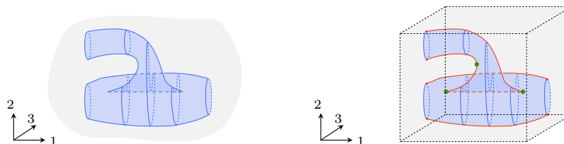
FIGURE 5.42. A tame tangle and a manifold diagram that refines it.
