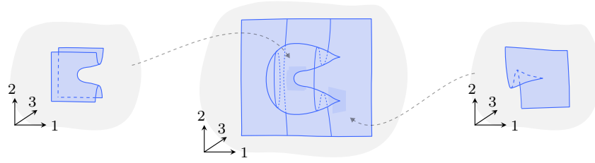
FIGURE 5.50. Tangle singularities in a tame 2-tangle.
