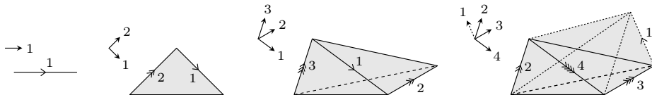
FIGURE 1.4. Framed simplices.
