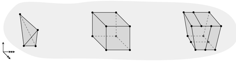
FIGURE 1.51. Framed 3-cells.
