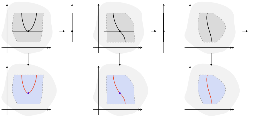
FIGURE 5.29. 2-Mesh singularities.
