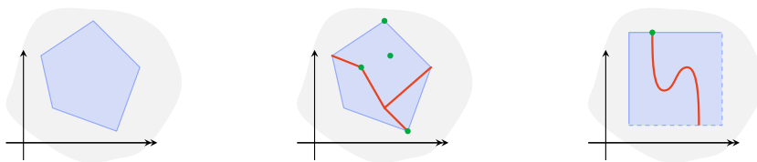
FIGURE 5.2. 2-Tame stratifications.
