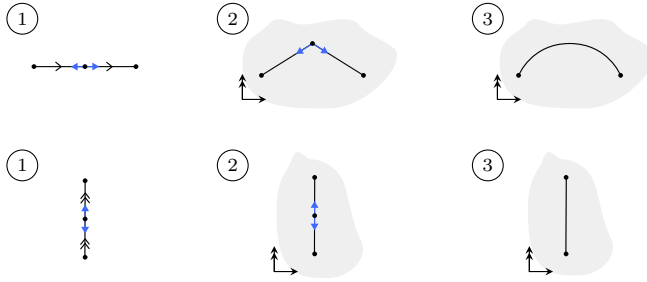
FIGURE 1.45. 2-Framed 1-cells.
