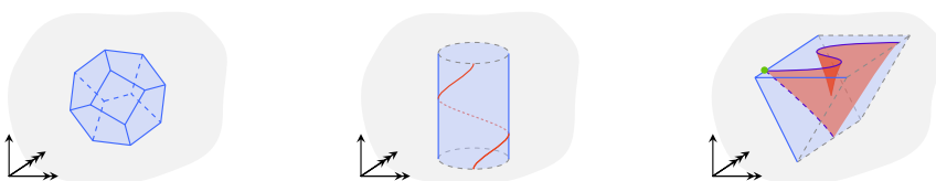
FIGURE 5.4. 3-Tame stratifications.
