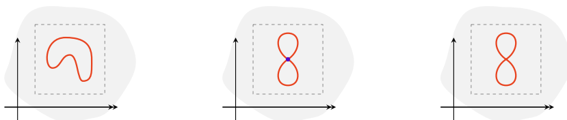
FIGURE 5.3. 2-Tame embeddings.
