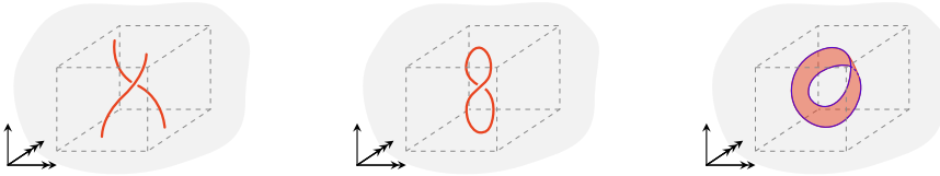
FIGURE 5.5. 3-Tame embeddings.
