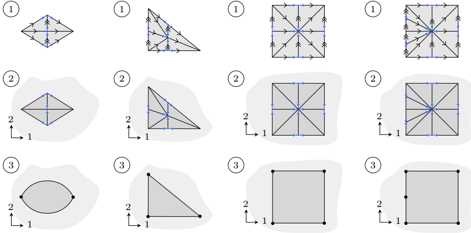
FIGURE 1.46. 2-Framed regular 2-cells.
