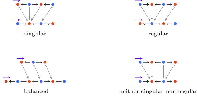
FIGURE 2.6. Types of maps of 1-trusses.
