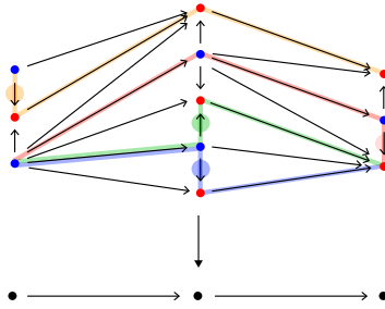
FIGURE 2.30. Spacers and their associated fiber morphisms.
