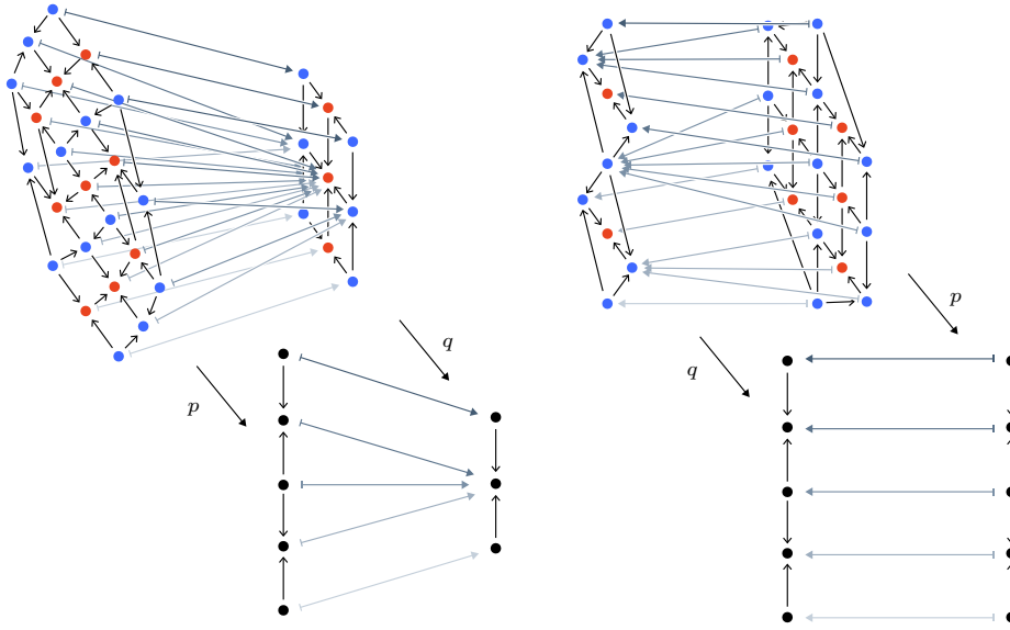
FIGURE 2.21. A singular and a regular 1-truss bundle map.
