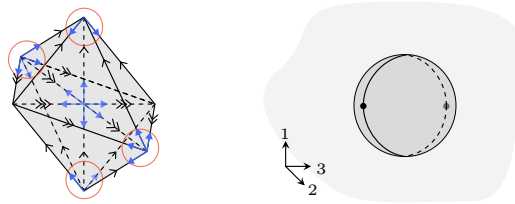
FIGURE 1.50. A framing of the simplicial complex underlying the regular 3-globe that is not a framed regular cell.
