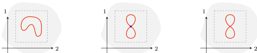
FIGURE 5.3. 2-Tame embeddings.
