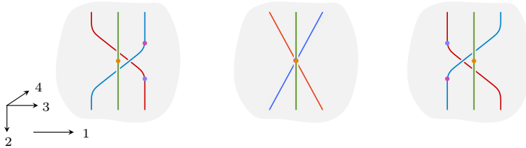
FIGURE 5.47. A manifold 3-diagram isotopy.
