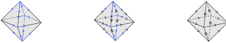
FIGURE 1.40. A 2-framed regular cell complex.
