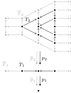
FIGURE 4.22. Cubical compactification of an open 2-truss.
