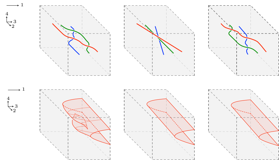
FIGURE I.7. Two tame stratifications of the 4-cube.
