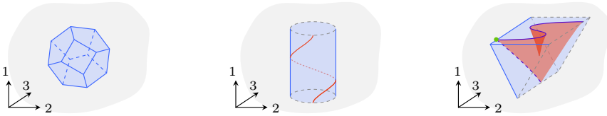
FIGURE 5.4. 3-Tame stratifications.
