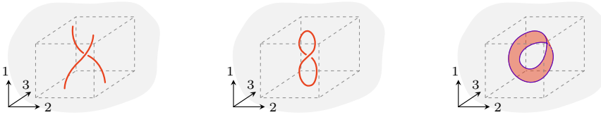
FIGURE 5.5. 3-Tame embeddings.
