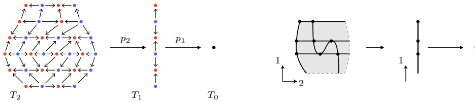
FIGURE 2.42. A 2-truss and corresponding stratifications.
