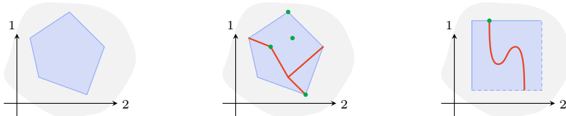
FIGURE 5.2. 2-Tame stratifications.
