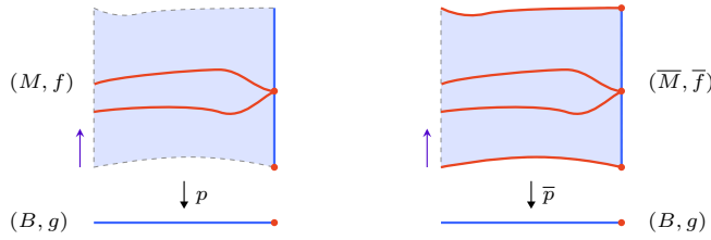
FIGURE 4.13. The compactification of a 1-mesh bundle.
