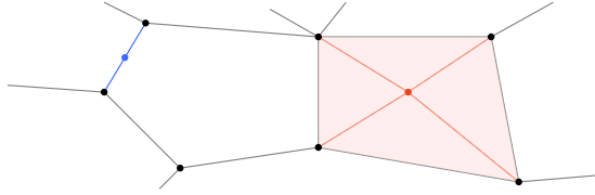
FIGURE B.16. The conical subdivision of a 1-cell (blue) and a 2-cell (red) in a regular cell complex.
