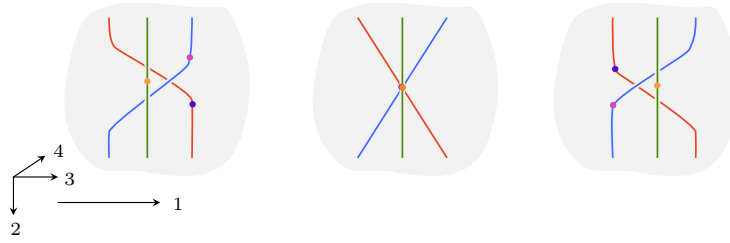
FIGURE 5.47. A manifold 3-diagram isotopy.
