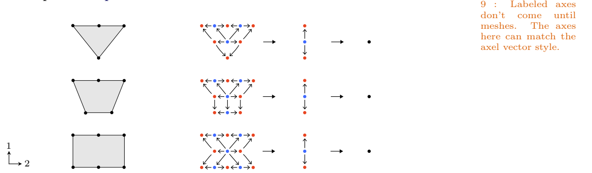
FIGURE I.3. Framed regular 2-cells and their truss blocks.
