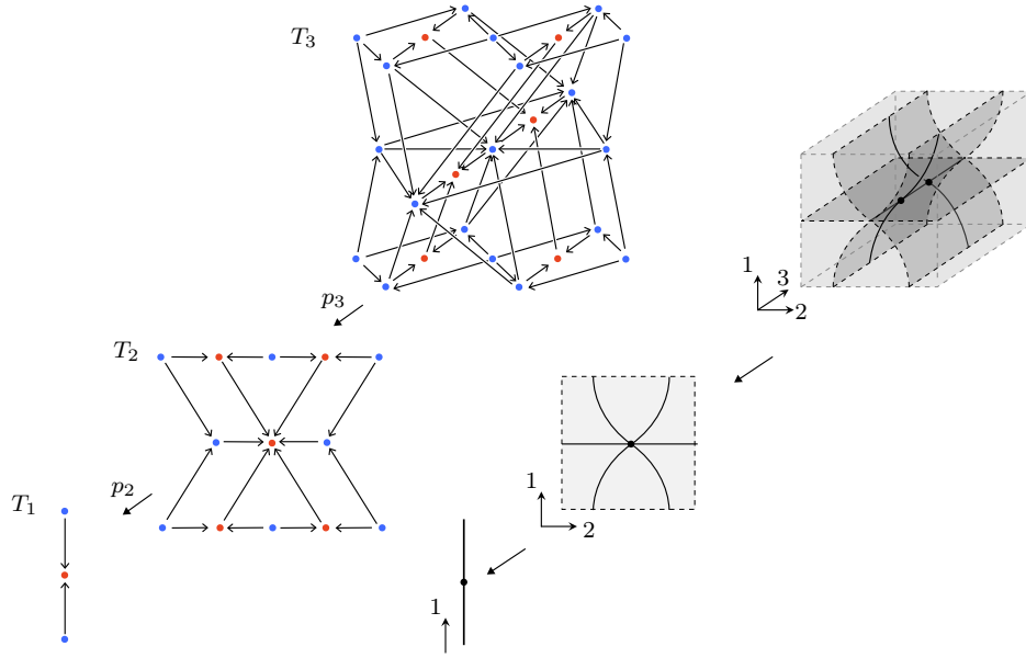
FIGURE 2.41. A 3-truss and its corresponding stratifications.
