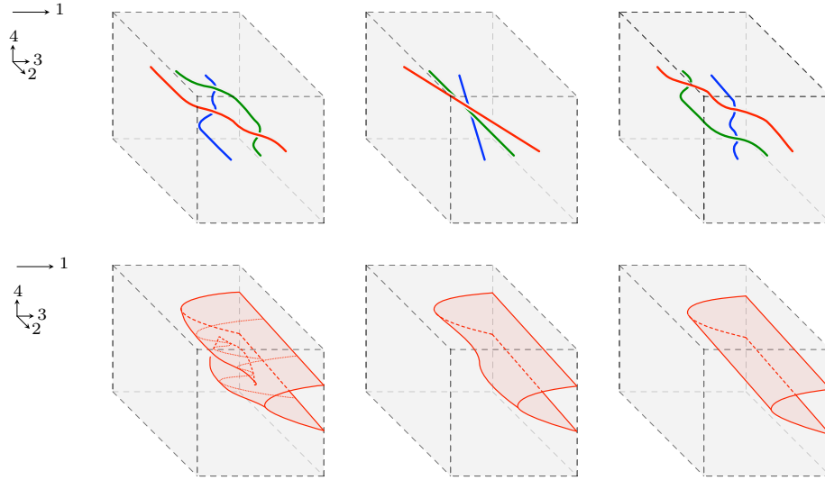
FIGURE I.9. A tame stratification with a swallowtail singularity.
