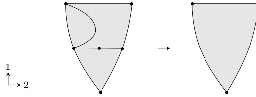
FIGURE I.6. A framed regular cell complex subdivision of a framed cell.
