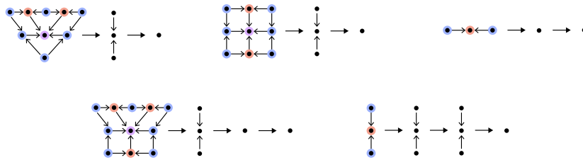
FIGURE 5.27. Truss singularities.
