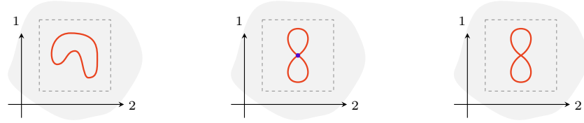
FIGURE 5.3. 2-Tame embeddings.
