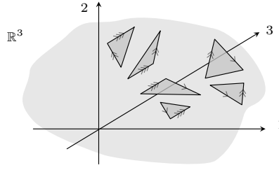
FIGURE 1.11. Framed realization of the 3-embedded framed 2-simplices.
