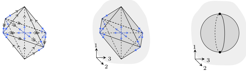
FIGURE 1.49. The simplest framed regular 3-cell.
