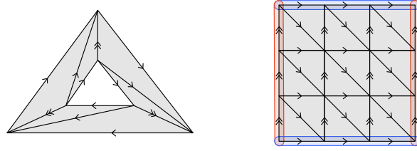
FIGURE 1.31. Progressive framed simplicial manifolds.
