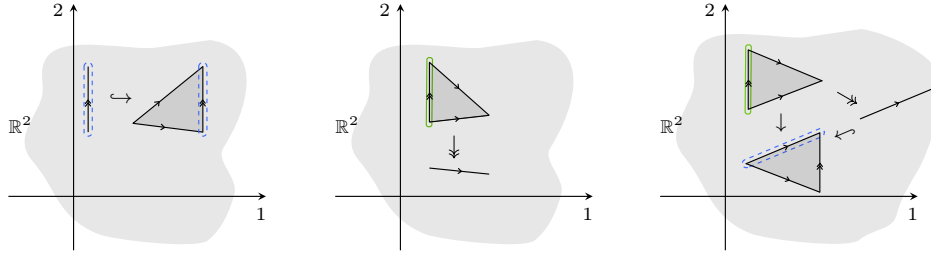
FIGURE 1.19. Framed maps via framed realization.
