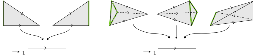
FIGURE 1.6. The 1-partially framed 2-simplices and 3-simplices.
