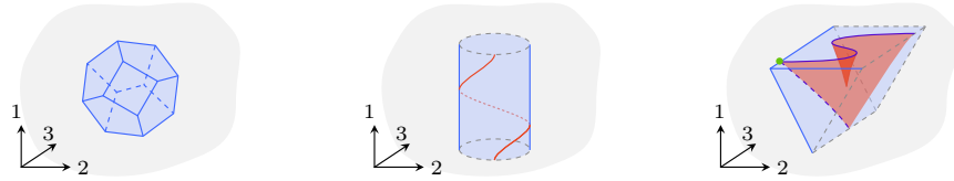
FIGURE 5.4. 3-Tame stratifications.
