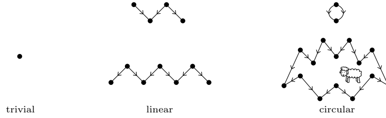
FIGURE 2.3. Fences of different types.
