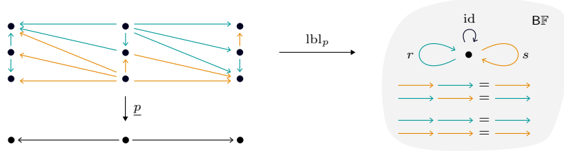
FIGURE 2.39. A 1-truss bundle labeled in a monoid.
