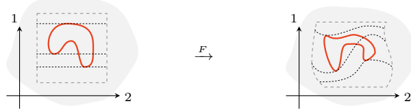
FIGURE 5.9. Non-framed stratified homeomorphism.
