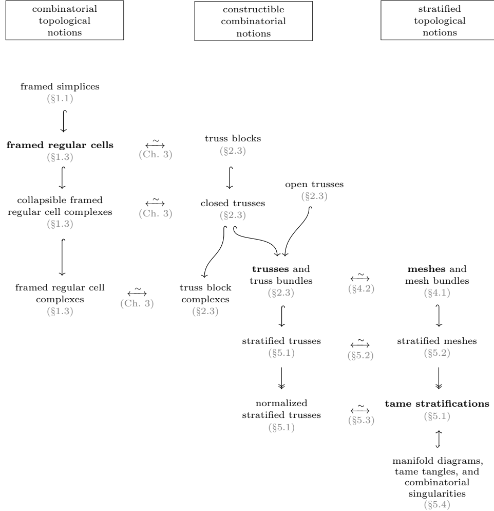
FIGURE I.11. Overview of concepts and connections.
