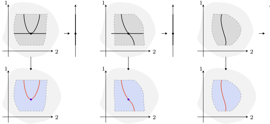
FIGURE 5.29. Mesh singularities.
