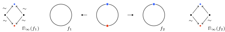
FIGURE B.17. Fundamental categories of two stratified circles.
