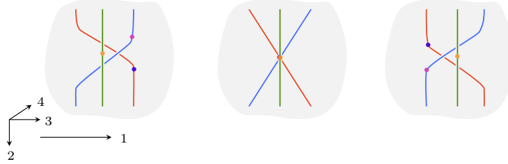
FIGURE 5.47. A manifold 3-diagram isotopy.
