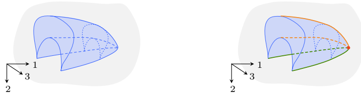
FIGURE 5.50. A projection of a 3-tangle singularity and its critical refinement.
