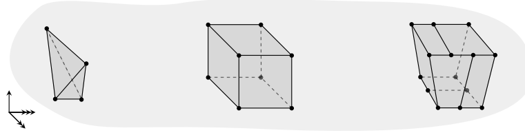
FIGURE 1.51. Framed 3-cells.
