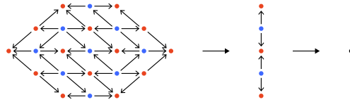
FIGURE I.2. A closed 2-truss.
