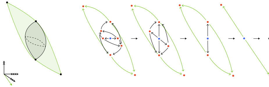
FIGURE B.7. The 4-globe as a framed 4-cell.
