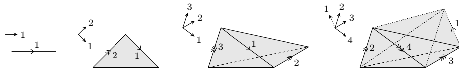
FIGURE 1.4. Framed simplices.
