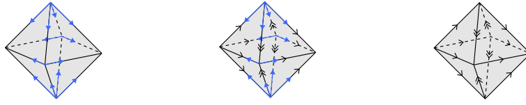
FIGURE 1.40. A 2-framed regular cell complex.
