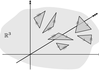
FIGURE 1.11. Framed realization of the 3-embedded framed 2-simplices.
