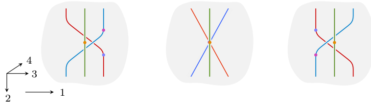
FIGURE 5.48. A manifold 3-diagram isotopy.
