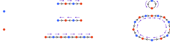
FIGURE 2.4. 1-Trusses of trivial, linear, and circular types.
