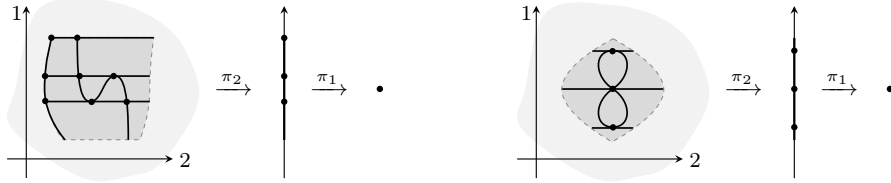
FIGURE 4.14. 2-Meshes with their framed realizations.
