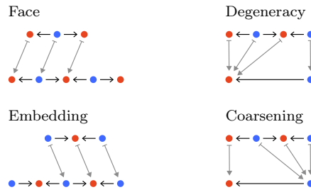
FIGURE 2.48. Face, embedding, degeneracy, and coarsening maps.
