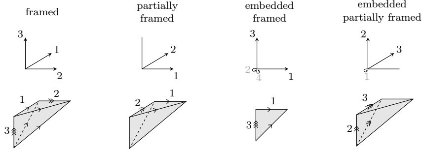
FIGURE 1.3. Frames on vector spaces and frames on simplices.
