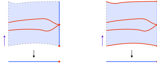
FIGURE 4.13. The compactification of a 1-mesh bundle.
