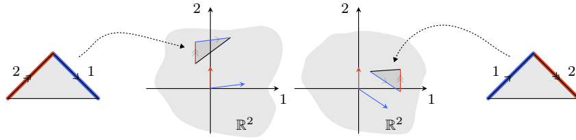
FIGURE 1.5. Framed realization of framed 2-simplices.
