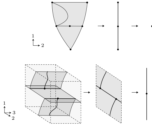
FIGURE I.4. A closed 2-mesh and an open 3-mesh.
