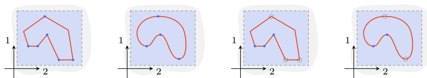
FIGURE 5.43. Framed conical and not framed conical stratifications.
