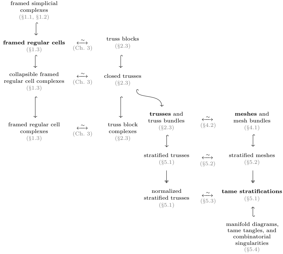
FIGURE I.11. Overview of concepts and connections.
