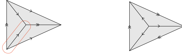
FIGURE 1.31. 2-Framed complexes which are not collapsible.
