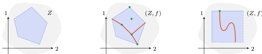
FIGURE 5.1. 2-Tame stratifications.
