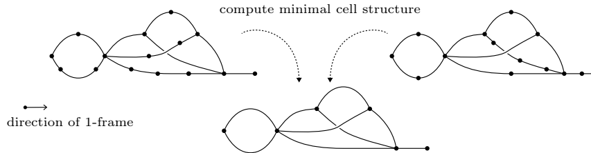
FIGURE 5.40. Decidability of framed homeomorphism for framed 1-complexes.
