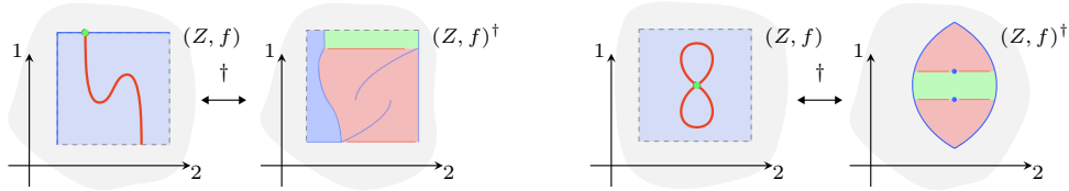
FIGURE 5.36. Duality of tame stratifications.
