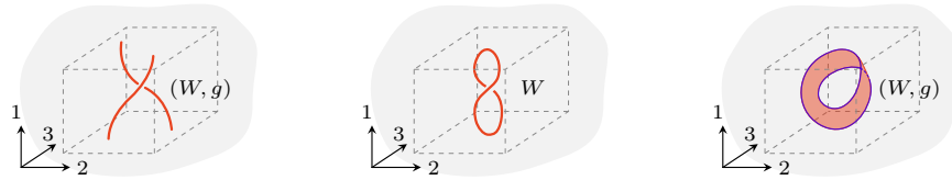
FIGURE 5.4. 3-Tame embeddings.
