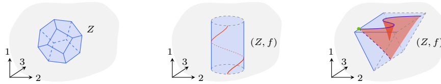
FIGURE 5.3. 3-Tame stratifications.
