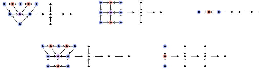
FIGURE 5.27. Truss singularities.
