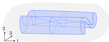
FIGURE 5.51. A 1-tangle isotopy.
