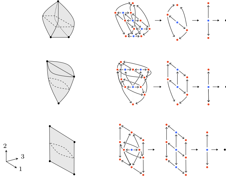
FIGURE I.4. Framed regular 3-cells and their classifying truss blocks.
