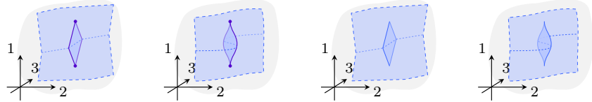
FIGURE 5.44. Framed conical and not framed conical embeddings.
