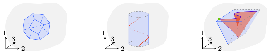
FIGURE 5.4. 3-Tame stratifications.
