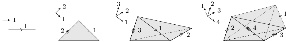
FIGURE 1.4. Framed simplices.
