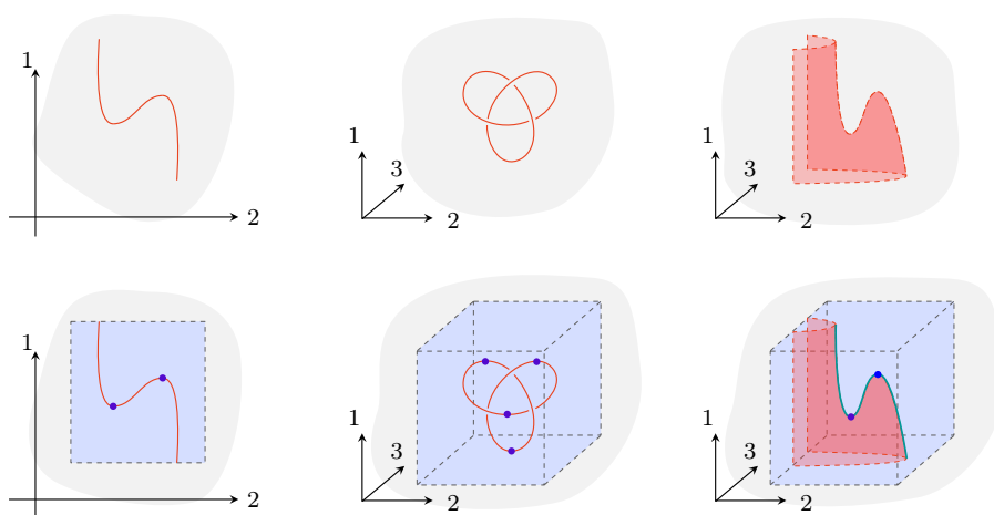
FIGURE 5.48. Tame tangles and their refining manifold diagrams.
