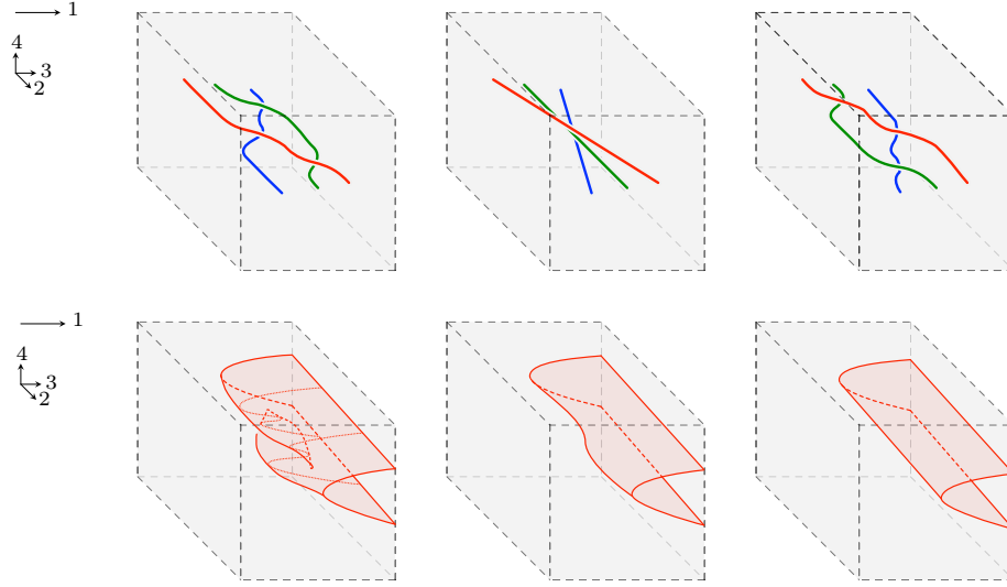
FIGURE I.8. Two tame stratifications of the 4-cube.
