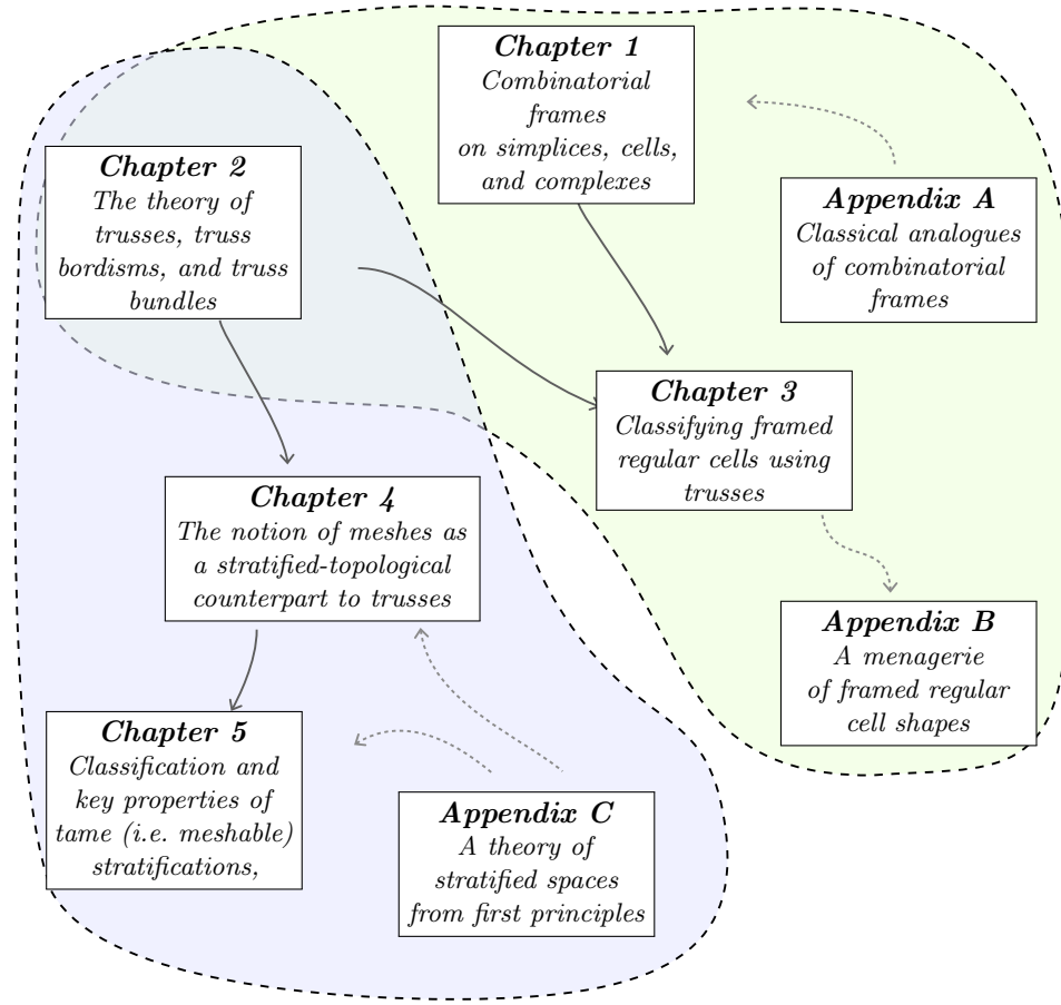
FIGURE I.13. Overview of dependencies.
