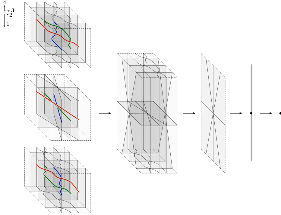
FIGURE I.10. The coarsest refining mesh of the third Reidemeister move.
