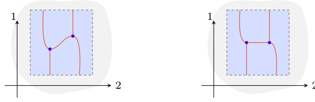
FIGURE 5.46. A manifold diagram and not a manifold diagram.
