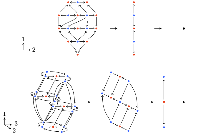
FIGURE I.2. A closed 2-truss and an open 3-truss.
