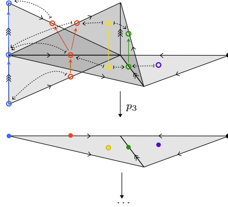
FIGURE 3.14. Fiber categories and transition functions.
