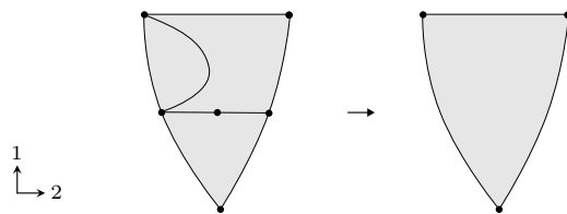
FIGURE I.6. A framed cell subdivision and a truss block subdivision.
