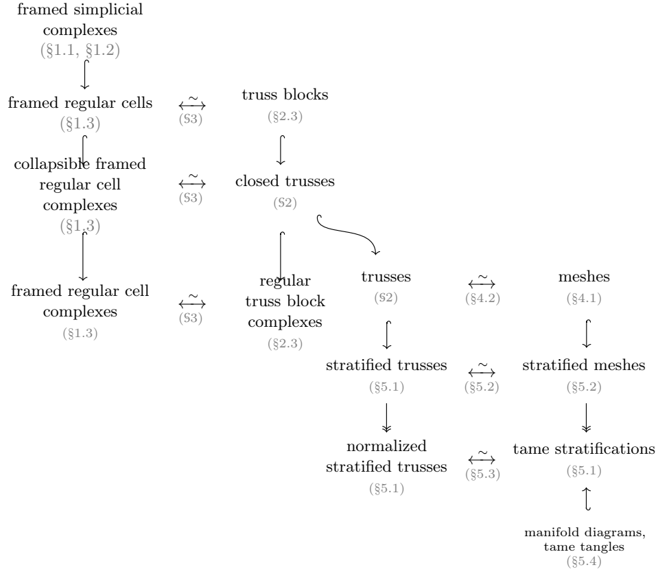
FIGURE I.12. Overview of concepts and connections.
