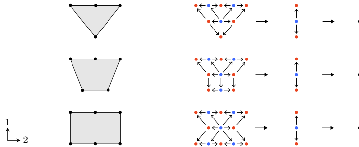
FIGURE I.3. Framed regular 2-cells and their classifying truss blocks.
