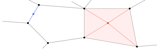
FIGURE C.16. The conical subdivision of a 1-cell (blue) and a 2-cell (red) in a regular cell complex.
