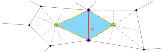
FIGURE C.15. The link (circled) and stratified cellular star (colored) of a cell x in a regular cell complex.
