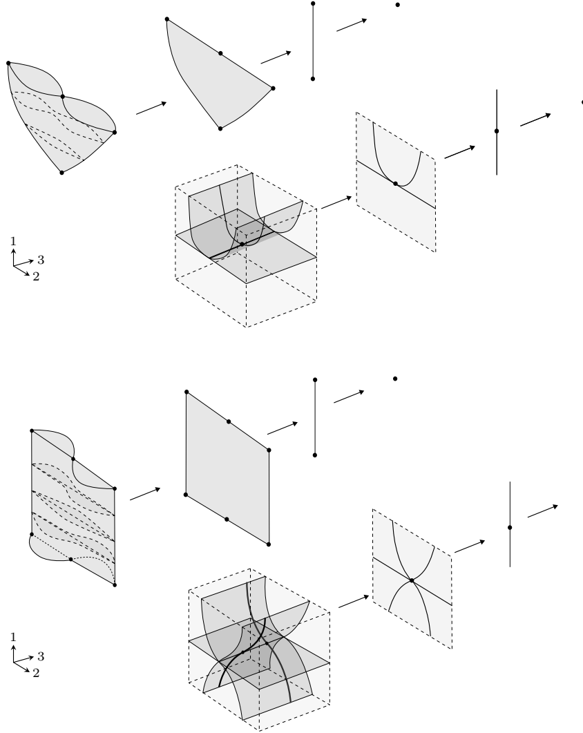
FIGURE I.7. Dualization of meshes.
