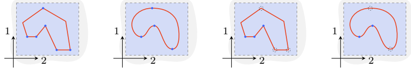
FIGURE 5.43. Framed conical and not framed conical stratifications.
