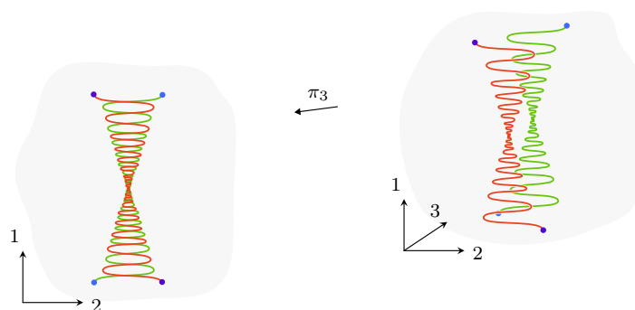
FIGURE 5.7. Nonlocal untameness.
